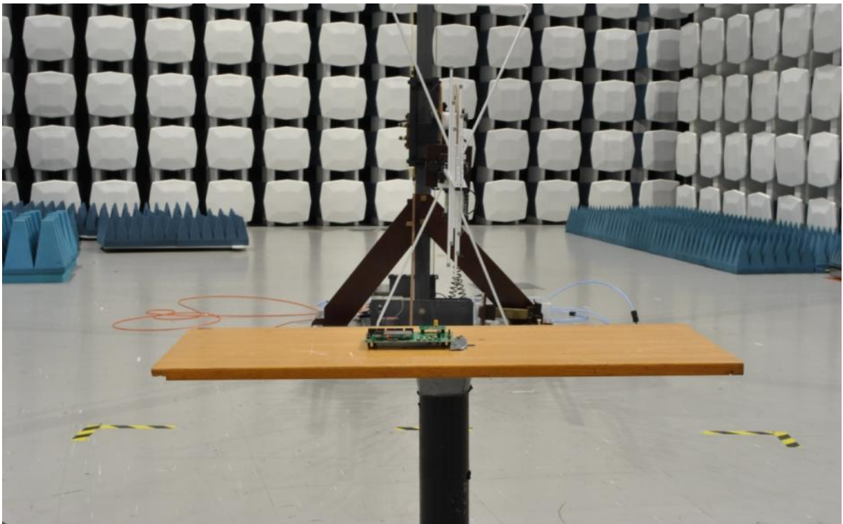
Radiated Emissions 30 - 1000 MHz, 3 meter
