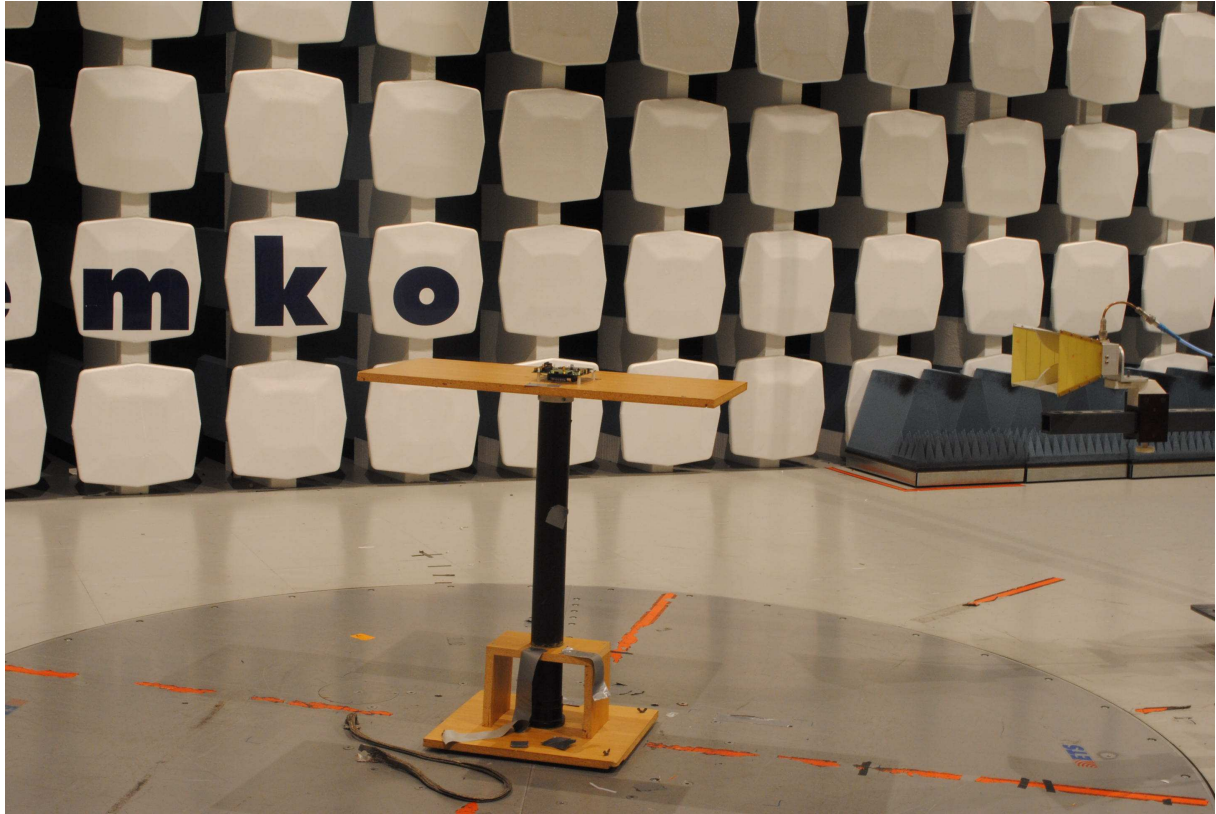
Radiated Emissions 12 - 25 GHz
