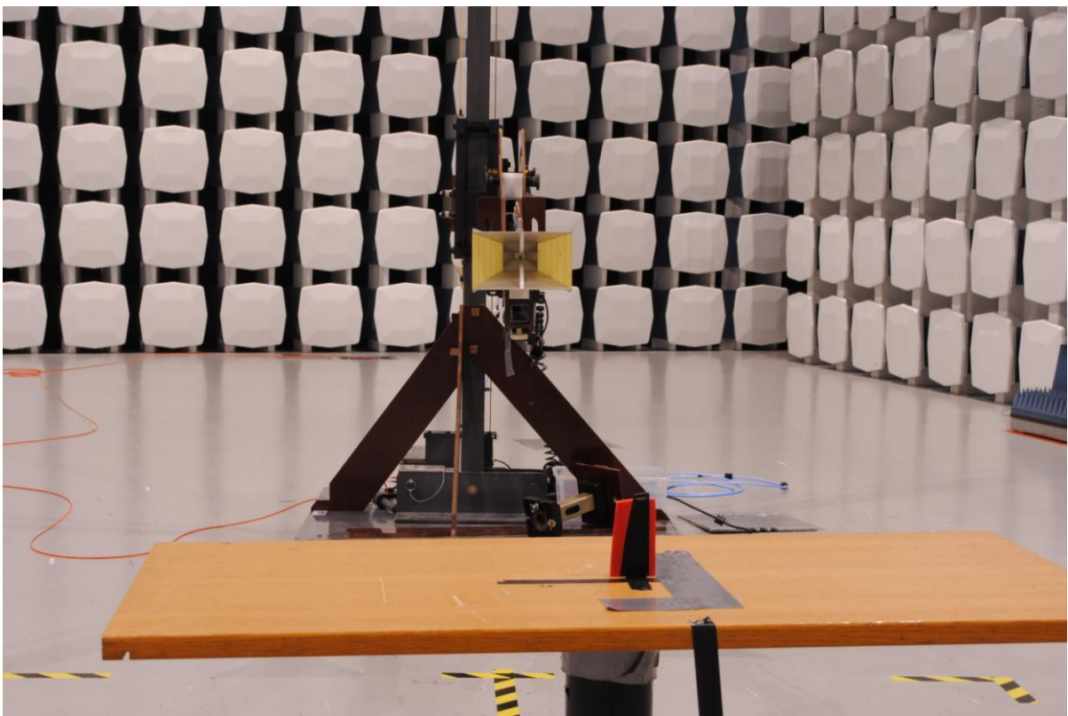
CC2541 SensorTag Radiated Emissions test (here with 1-18 GHz antenna shown)
