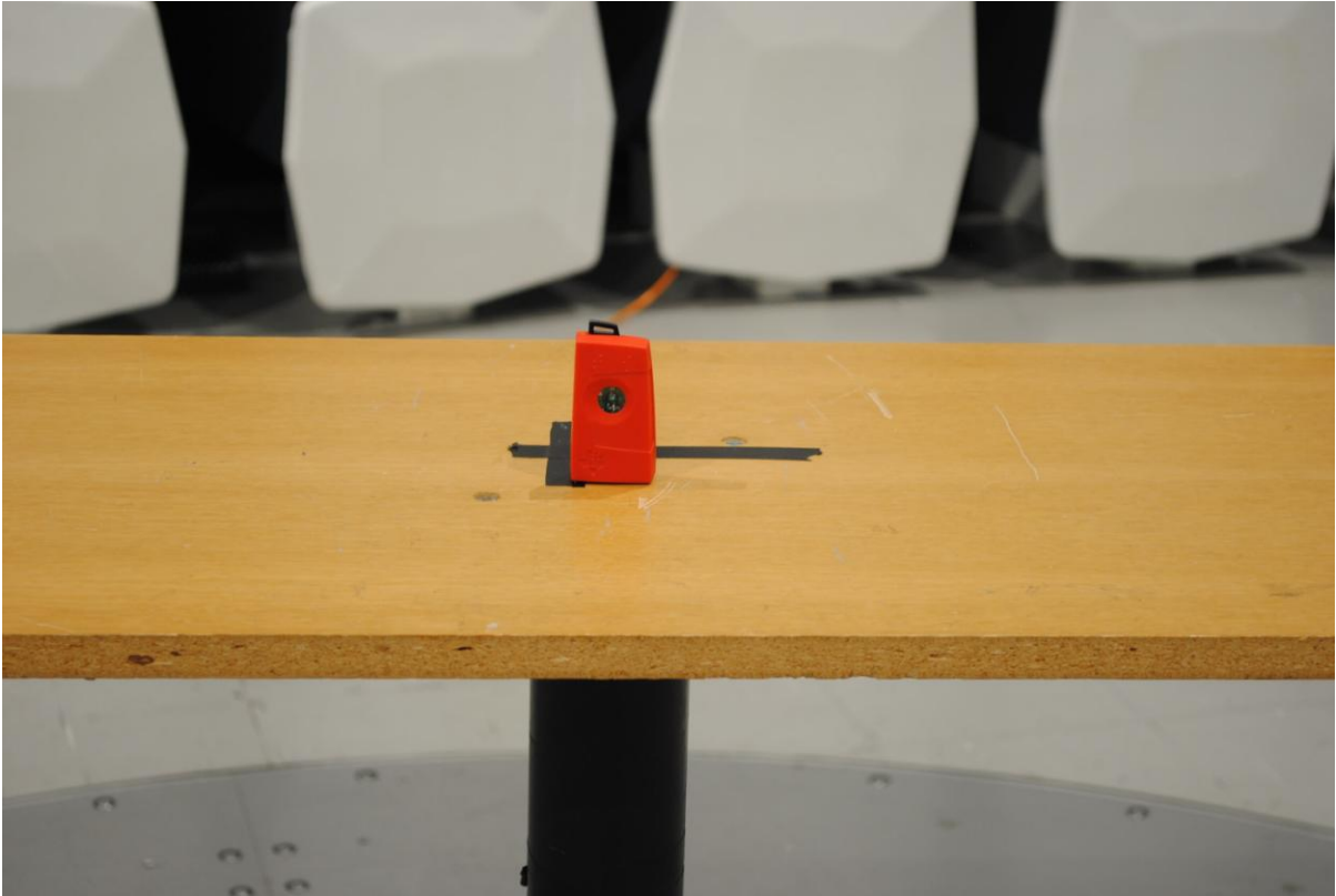
CC2541 SensorTag Radiated Emissions test
