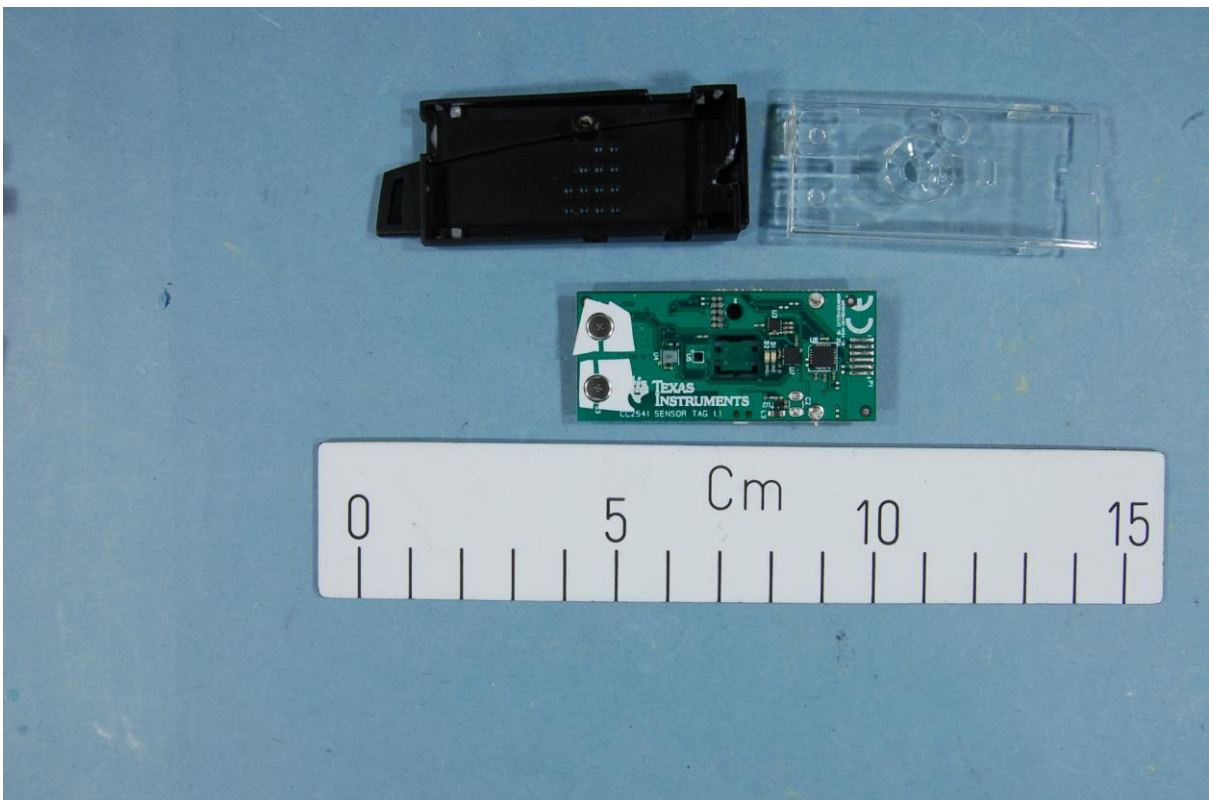
CC 2541 SensorTag de-assembled
