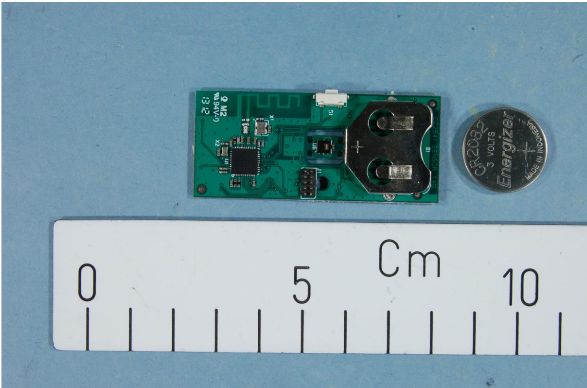
CC 2541 SensorTag PCB
