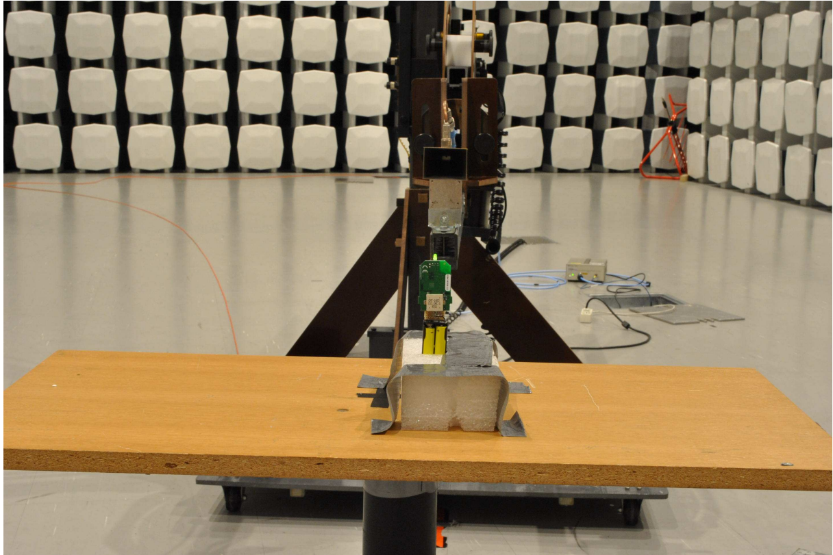
Radiated Emissions 12 - 18 GHz, 1 meter
