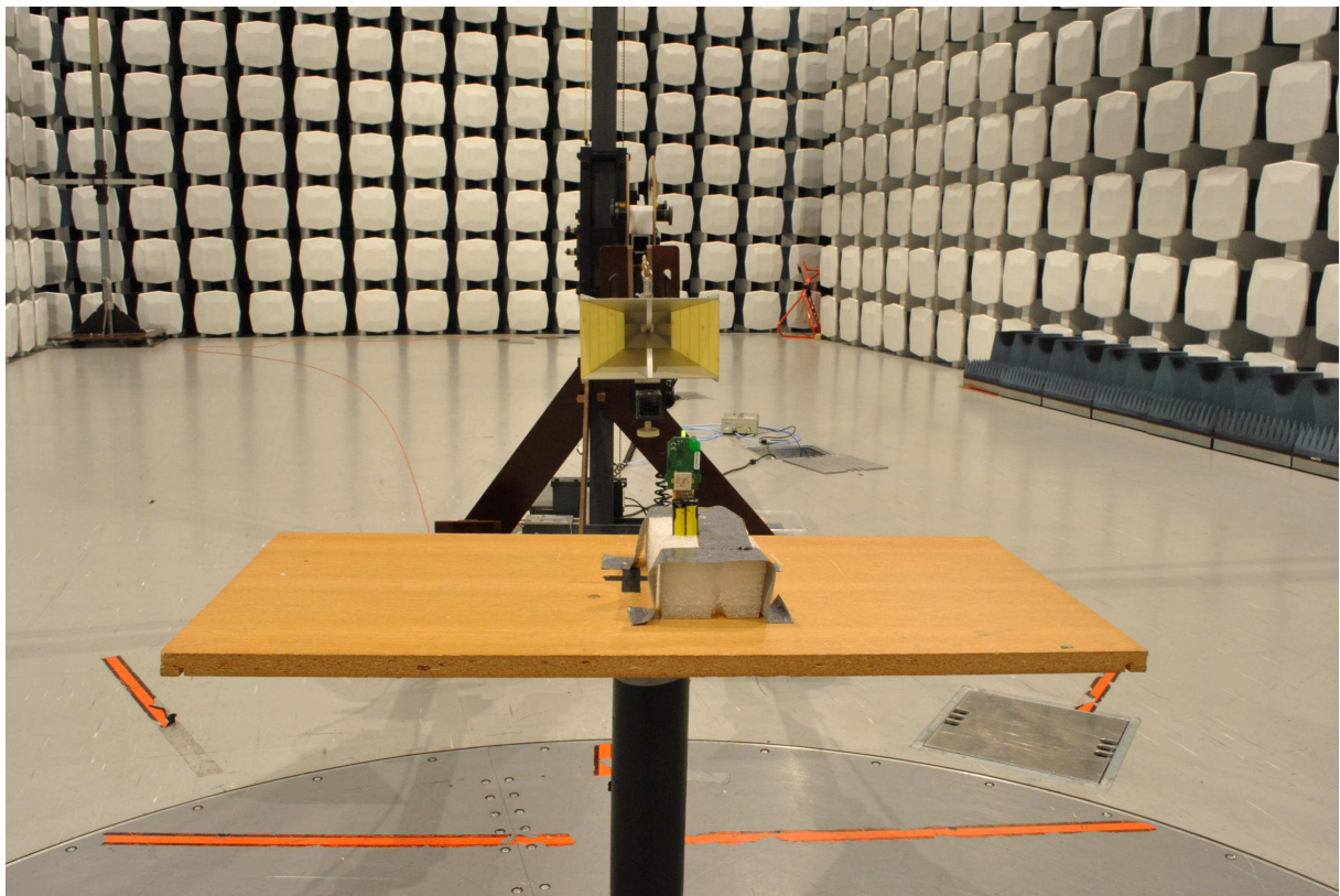
Radiated emissions 1 - 12 GHz, 3 meter
