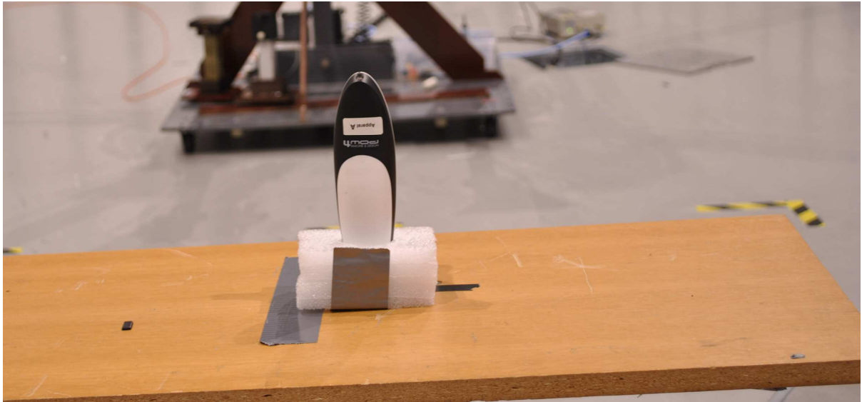
XY plane - Radiated Emissions
