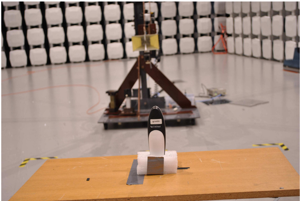
Radiated emissions 1 - 8.5 GHz, 3 meter
