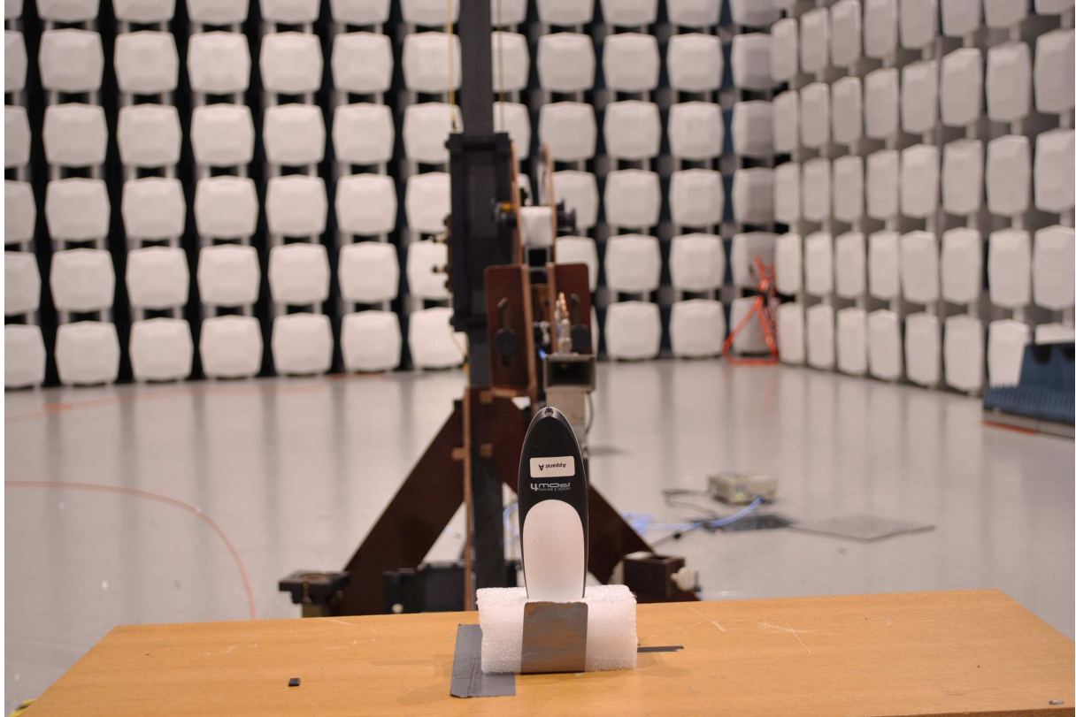
Radiated Emissions 8.5 - 12 GHz, 1 meter
