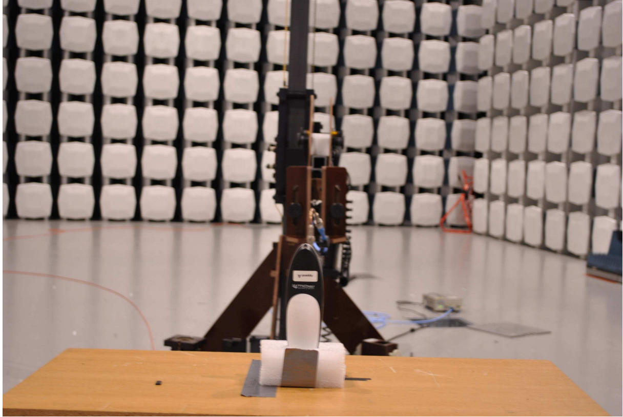
Radiated Emissions 18 - 25GHz, 1 meter
