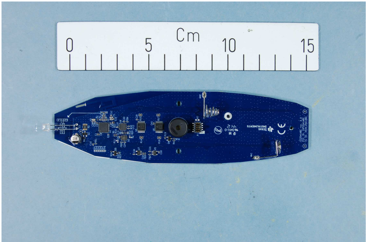
CC2541ARC, EUT for radiated measurements
