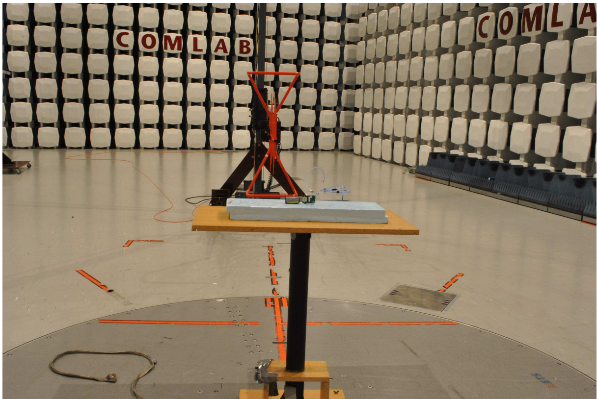
YZ plane - Radiated Emissions
