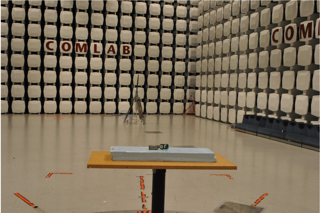
Radiated emissions - < 30MHz
