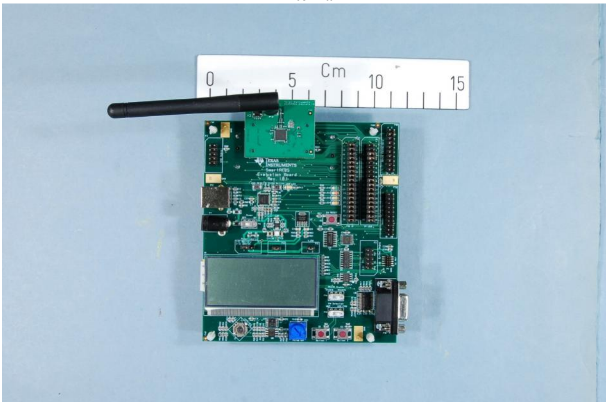
CC2540EM with evaluation board SmartRF05EB
