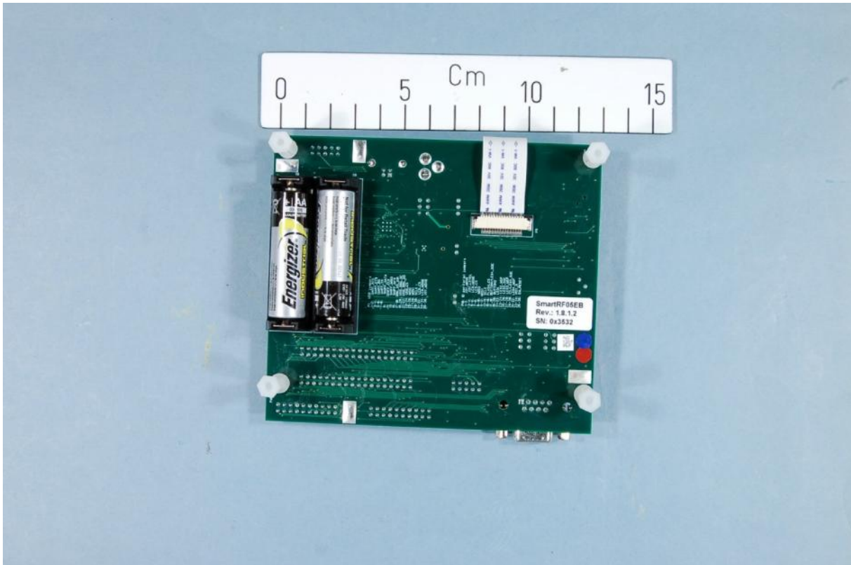
evaluation board SmartRF05EB-rear side with 2xAA batteries
