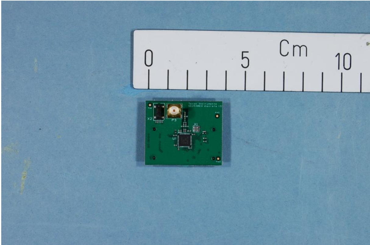
CC2540EM – PCB component side
