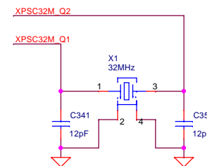
32 MHz crystal
