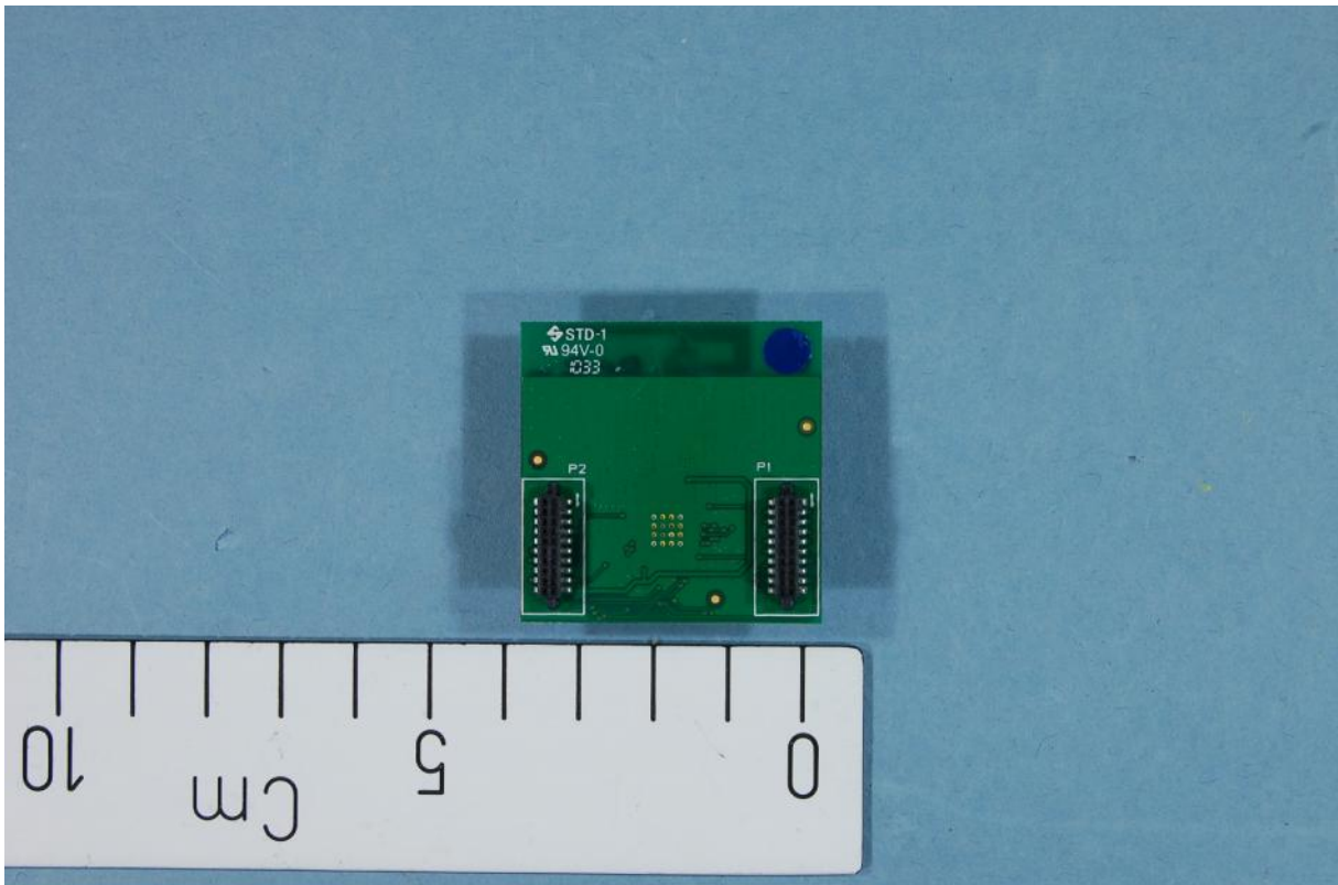
CC2433EM, EUT for radiated measurements
