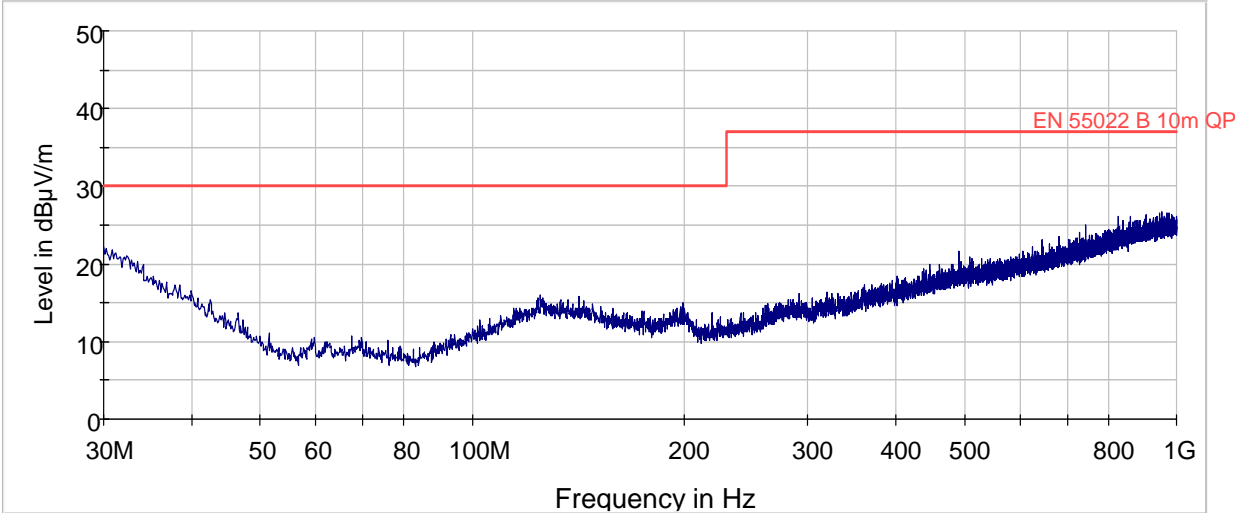
Radiated Emissions, 30 – 1000 MHz, VP and HP, @10m
