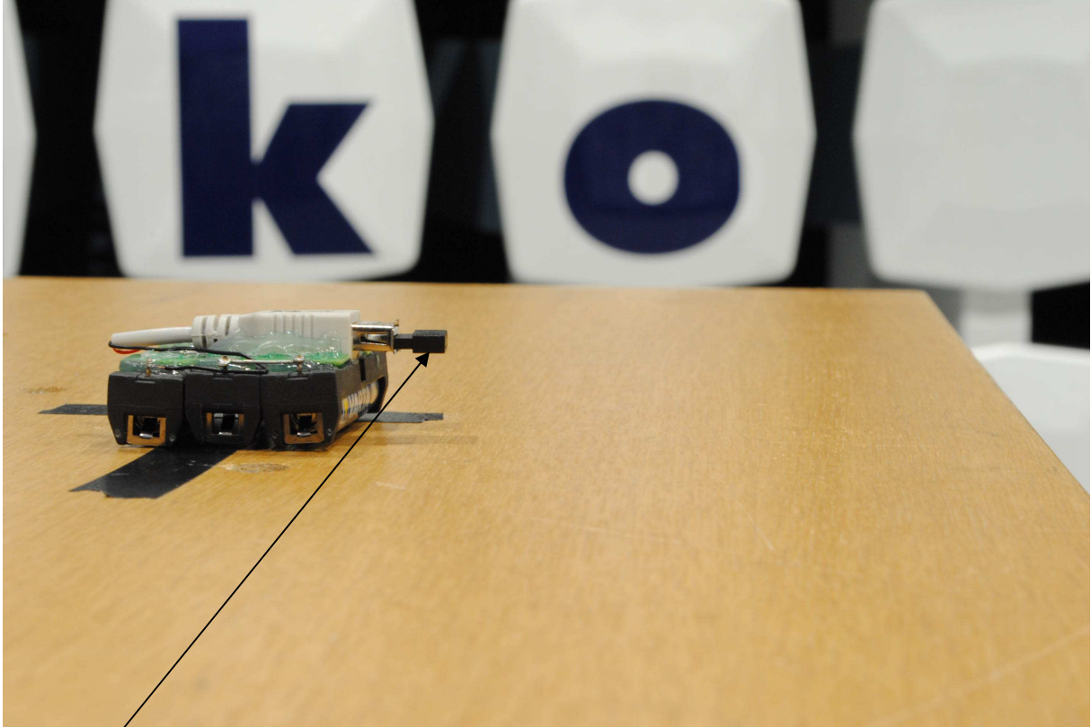
Radiated emission 9kHz - 25GHz CC2531
