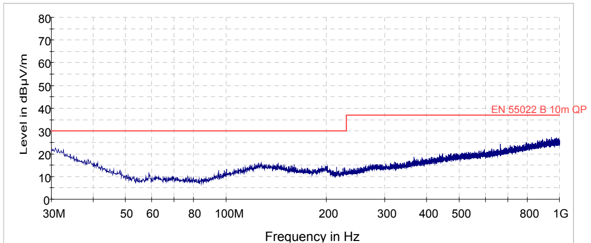
Radiated Emissions, 30 – 1000 MHz, VP and HP, @10m
