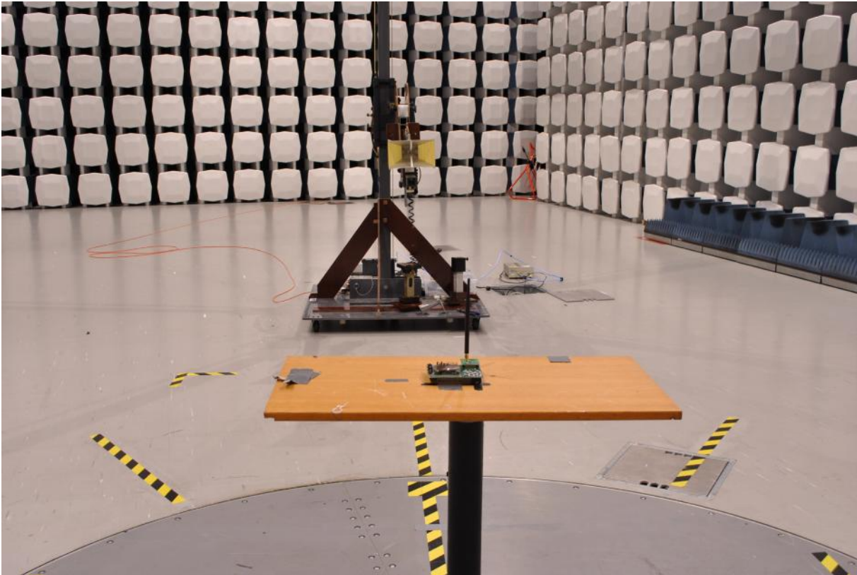
Radiated emissions >1 GHz
