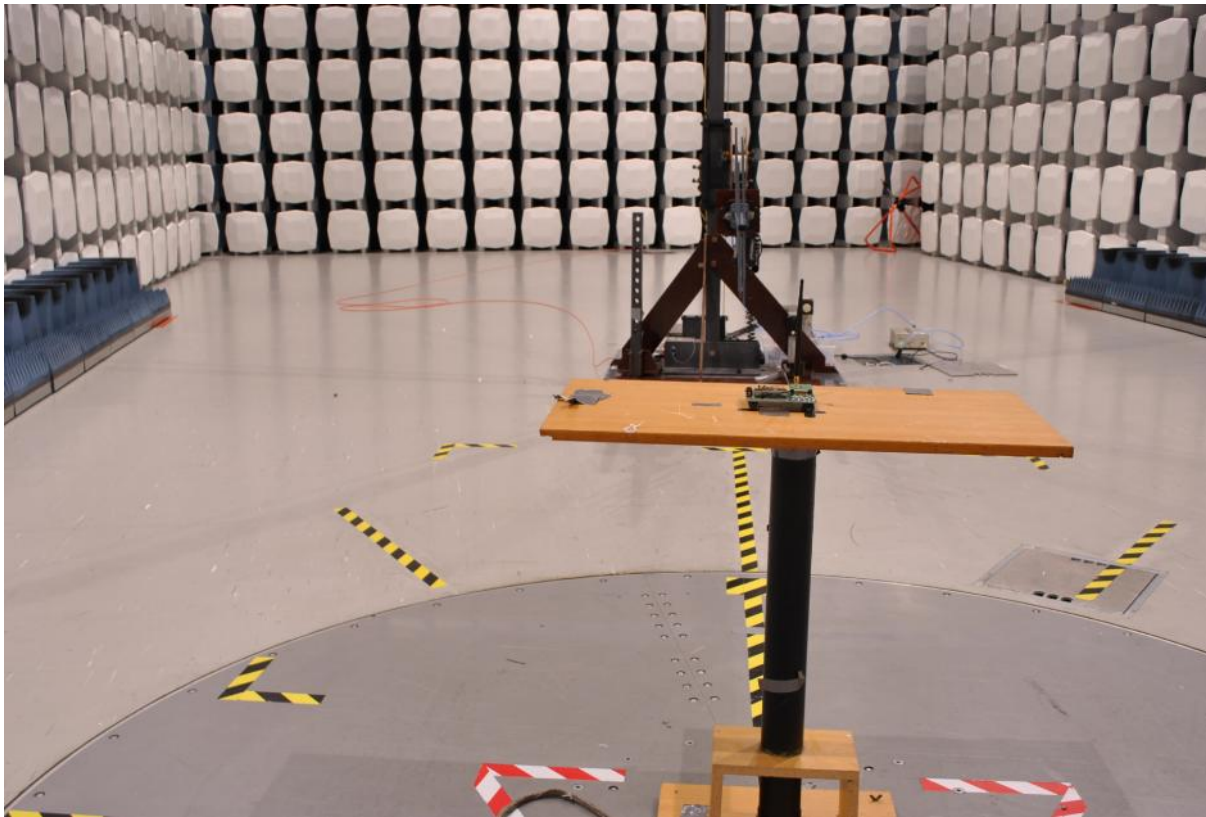
Radiated emissions - In band – VP
