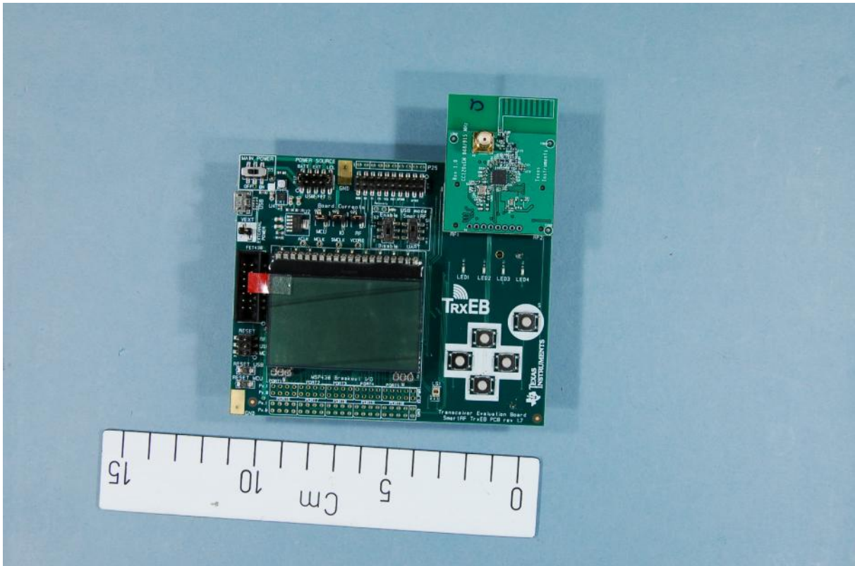
CC1200EM-868-930 hosted on TrxEB
