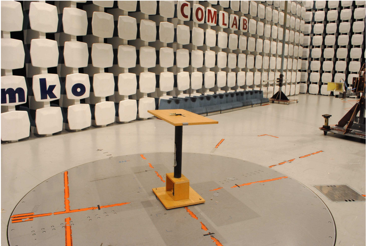
Radiated Emissions Test – 1 - 10GHz
