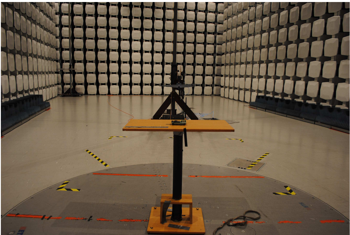
Radiated emissions – In band – HP
