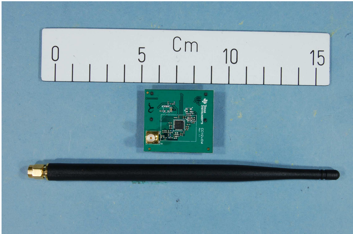
CC1175EM with the W5017 antenna
