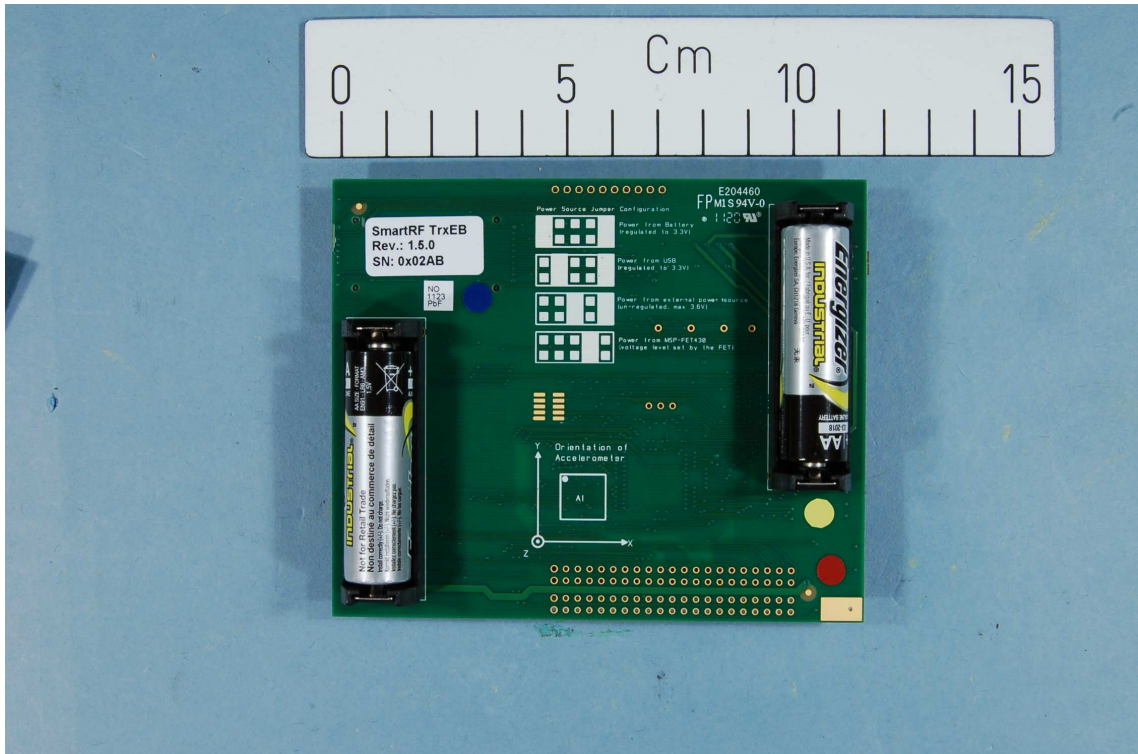
TrxEB with 2xAA Batteries
