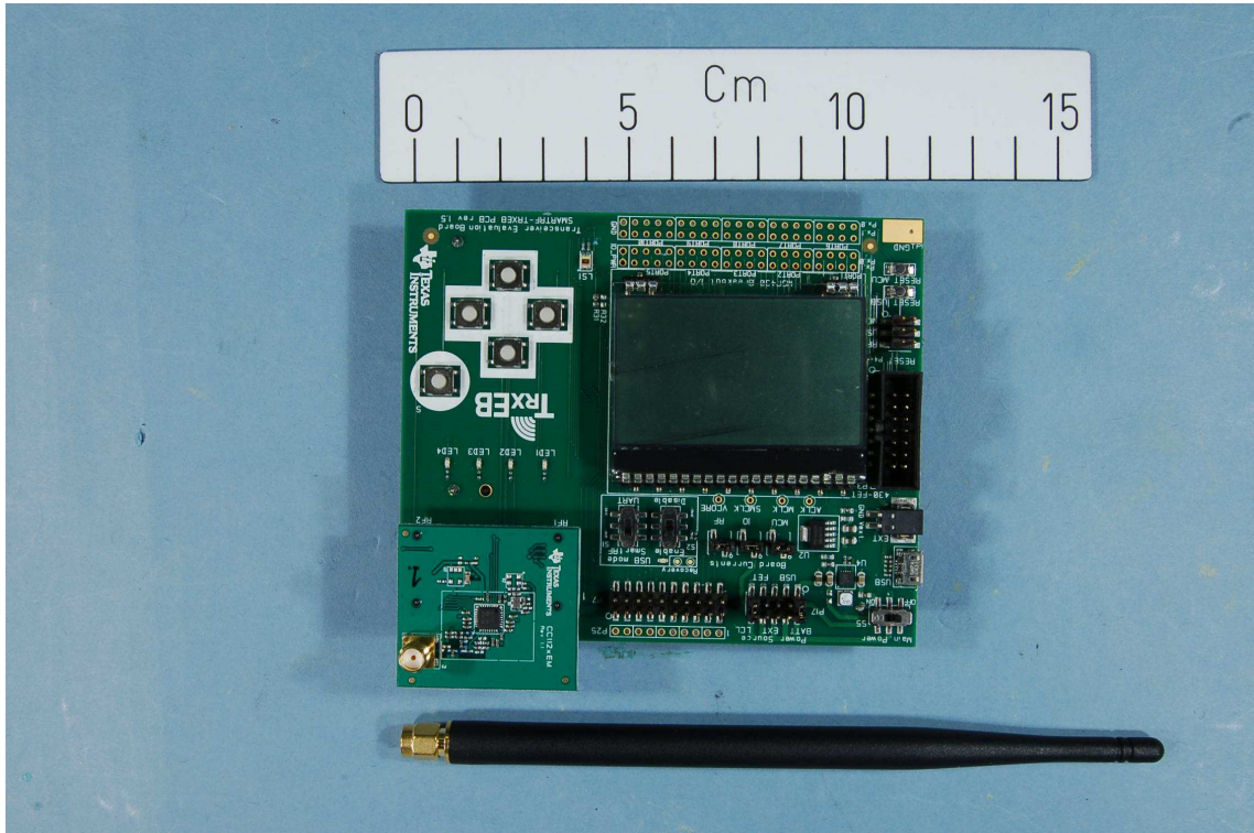
CC1175EM docking on TrxEB
