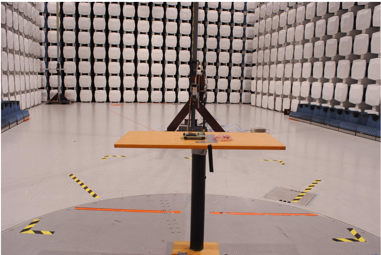
Radiated emissions > 8.5 GHz
