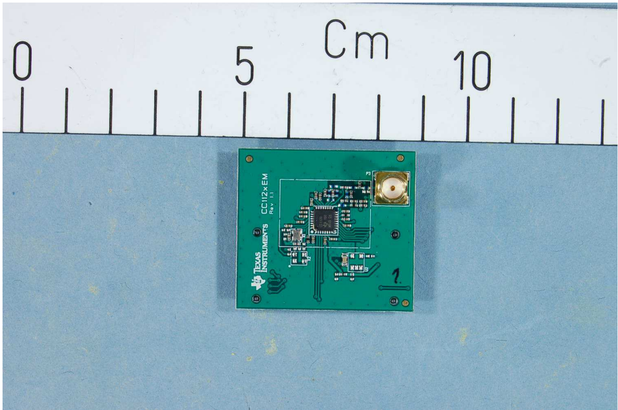
CC1120EM-868-915 with the W5017 antenna
