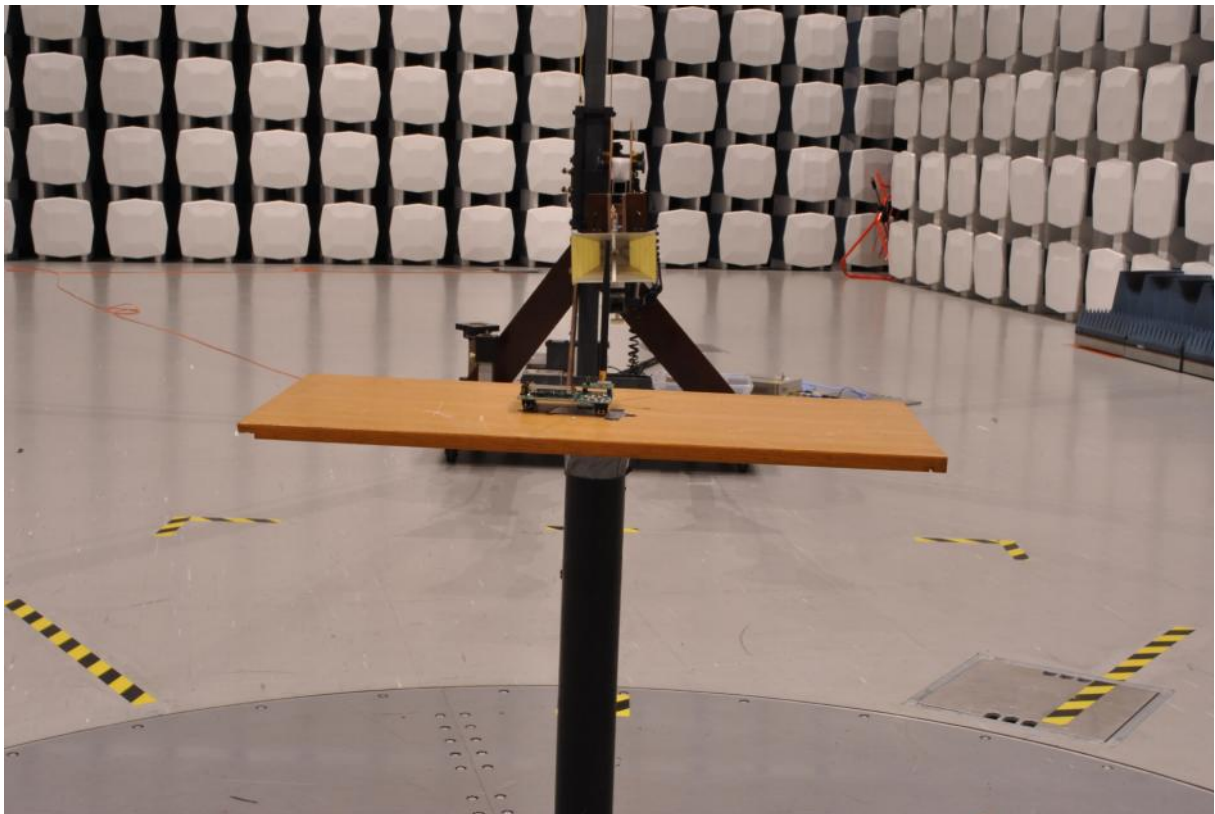
Radiated emissions 1 - 10 GHz, 3 meter
