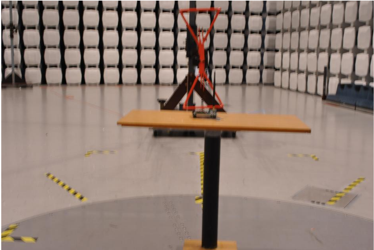
Radiated Emissions 30 - 902 & 902 - 1000 MHz, 3 meter
