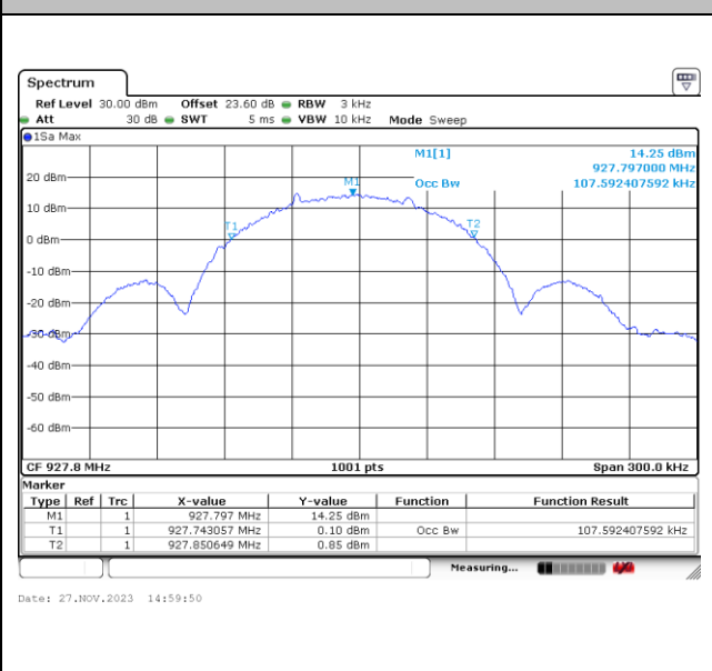
99% Occupied Bandwidth on Channel 129
