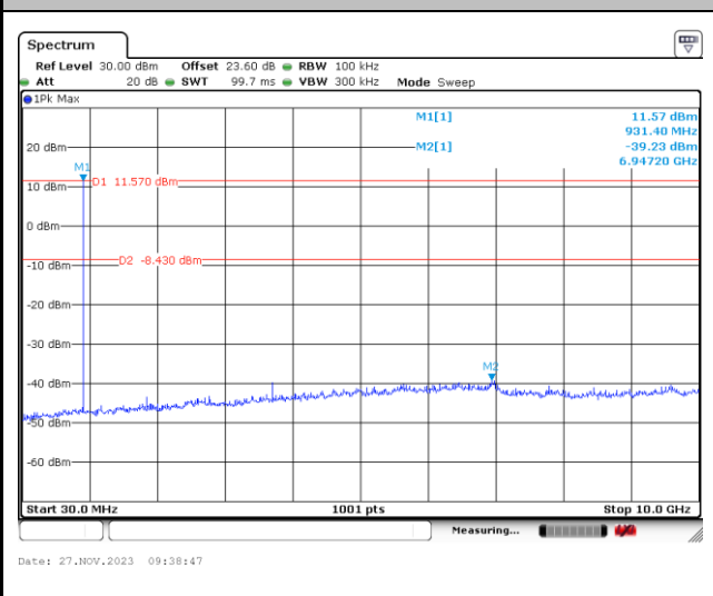
CSE Plot on Ch 129 between 30MHz ~ 10 GHz
