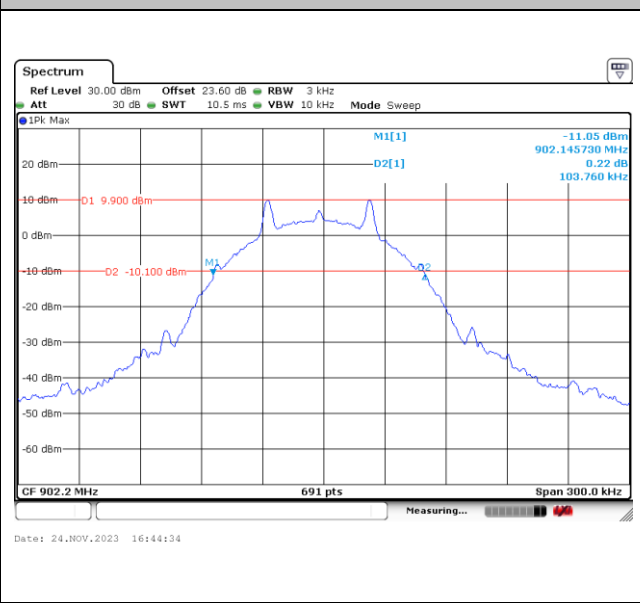
20 dB Bandwidth Plot on Channel 129
