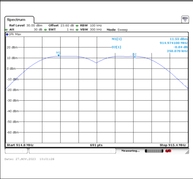
Channel Separation Plot on Channel 65 - 66
