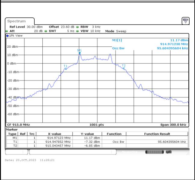
99% Occupied Bandwidth on Channel 65
