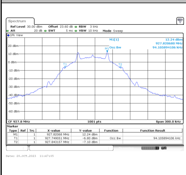
99% Occupied Bandwidth on Channel 129
