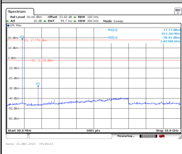
CSE Plot on Ch 65 between 30MHz ~ 10 GHz
