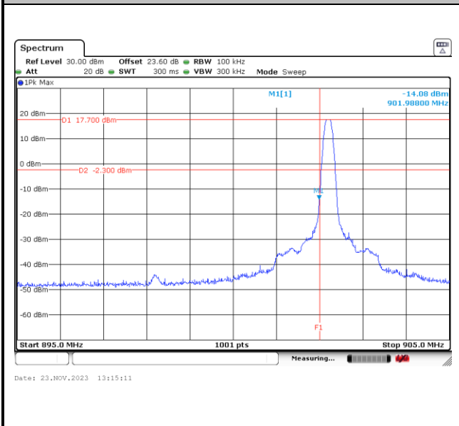
Low Band Edge Plot on Channel 101
