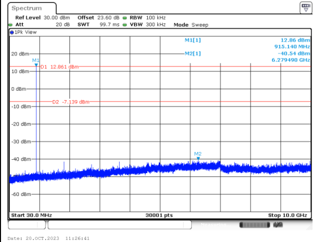
CSE Plot on Ch 65 between 30MHz ~ 10 GHz
