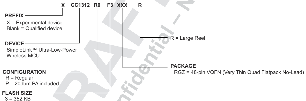
Figure 12-1. Device Nomenclature
