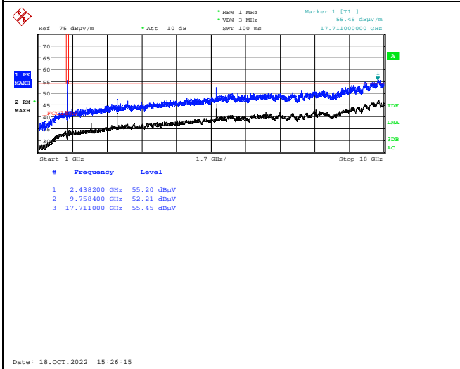
Radiated Emissions 1 - 18 GHz, 2440 MHz, 1Mb, HP
