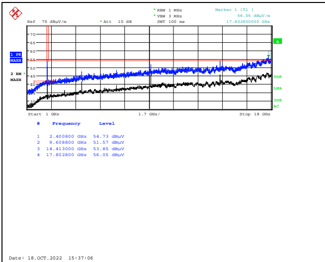
Radiated Emissions 1 - 18 GHz, 2402 MHz, 1Mb, HP
