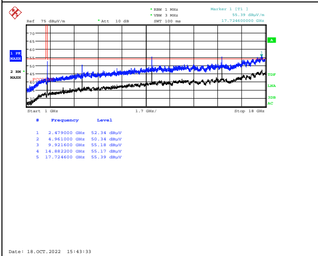
Radiated Emissions 1 - 18 GHz, 2480 MHz, 1Mb, HP
