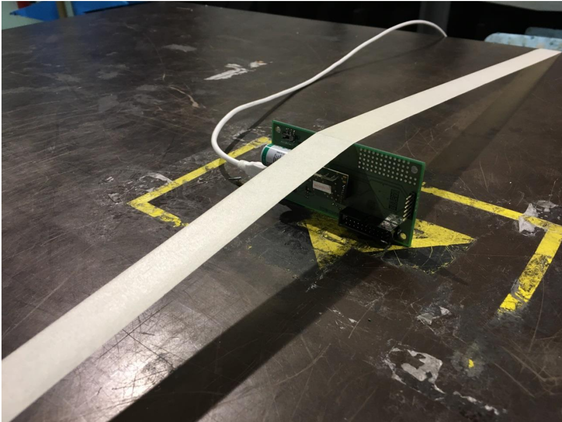
Test set up of EUT during radiated emission 30 – 1000 MHz
