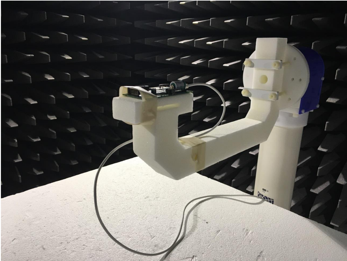
Test set up of EUT during radiated emission above 1 GHz
