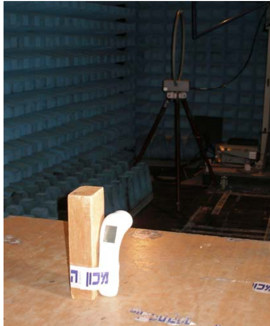
Photo 3. RE test setup in Anechoic chamber.
