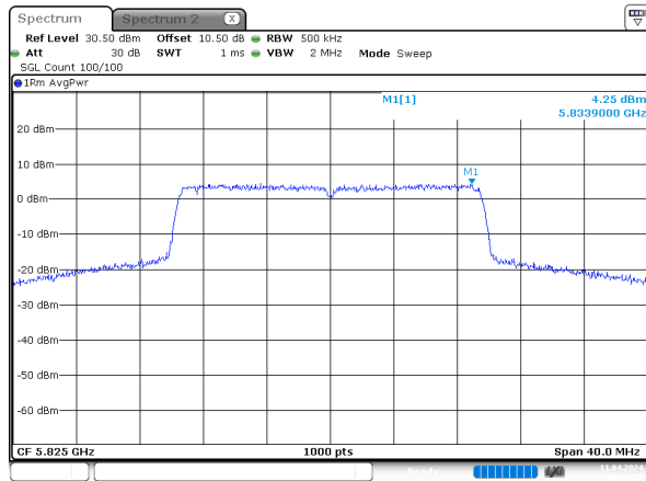
ax20_5825MHz_RU_Full_Chain 0
