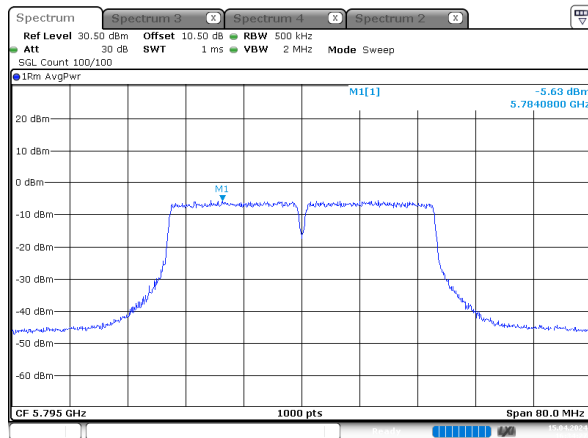
n40_5795MHz_Chain 2
