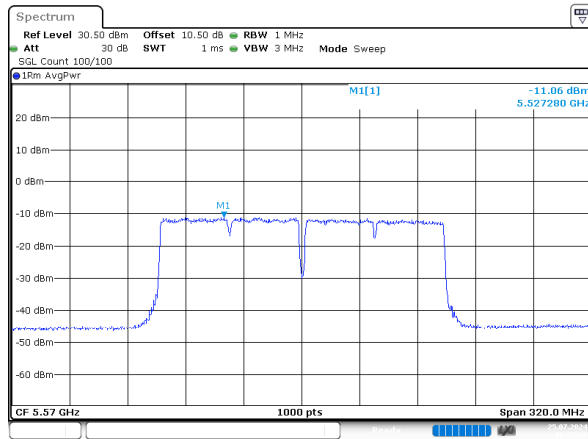
ac160_5570MHz_Chain 0
