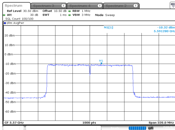
ax160_5570MHz_RU_Full_Chain 2
