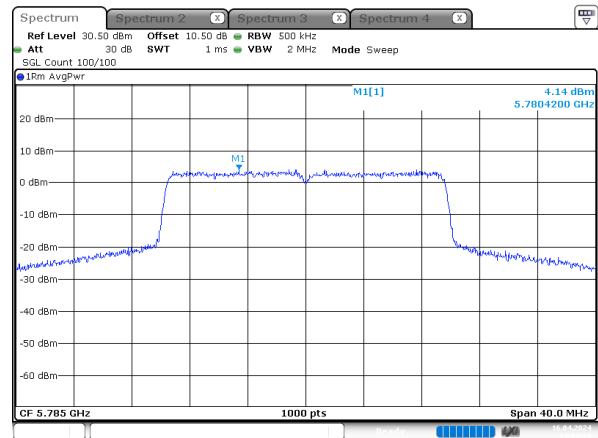
ax20_5785MHz_RU_Full_Chain 3
