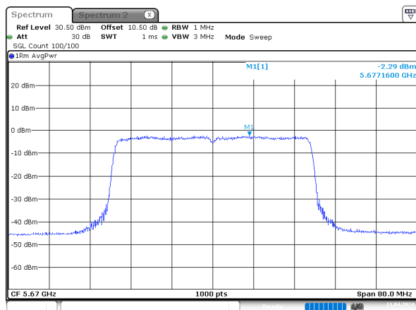
ax40_5670MHz_RU_Full_Chain 0
