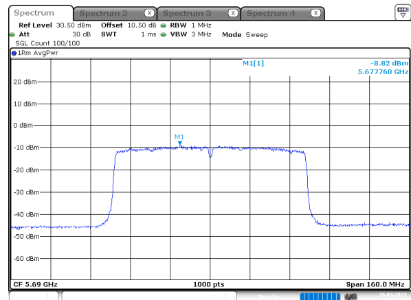
ac80_5690MHz_Chain 3
