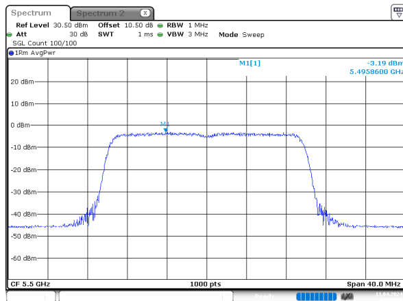
ax20_5500MHz_RU_Full_Chain 0
