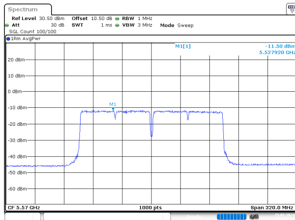
ac160_5570MHz_Chain 2
