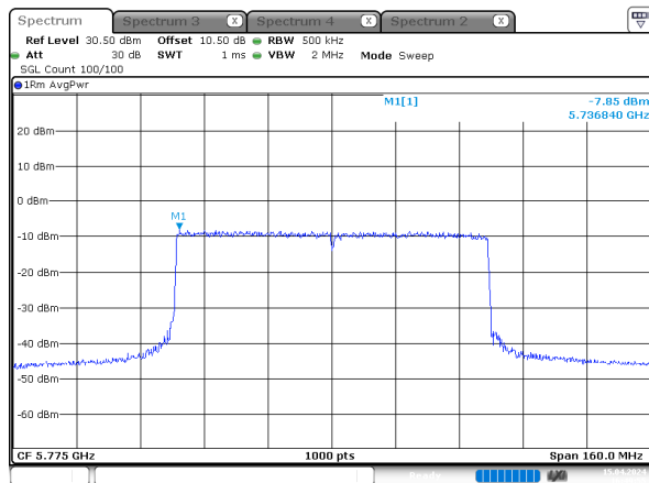
ax80_5775MHz_RU_Full_Chain 2
