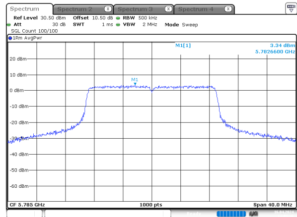
n20_5785MHz_Chain 3
