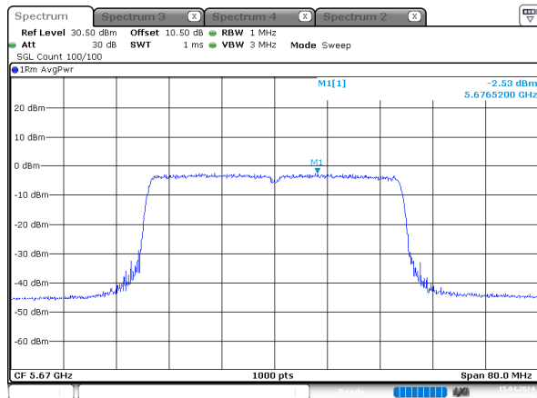
ax40_5670MHz_RU_Full_Chain 2
