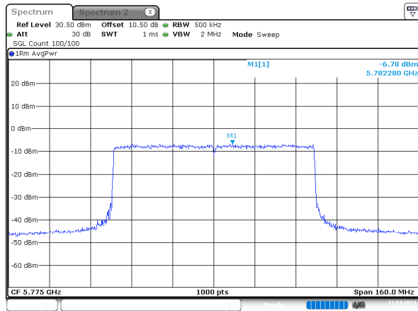
ax80_5775MHz_RU_Full_Chain 0
