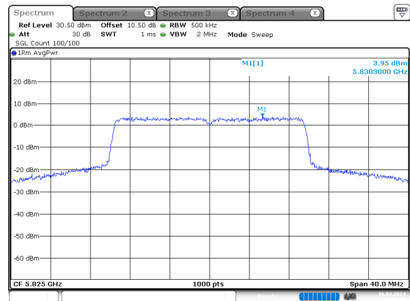
ax20_5825MHz_RU_Full_Chain 3
