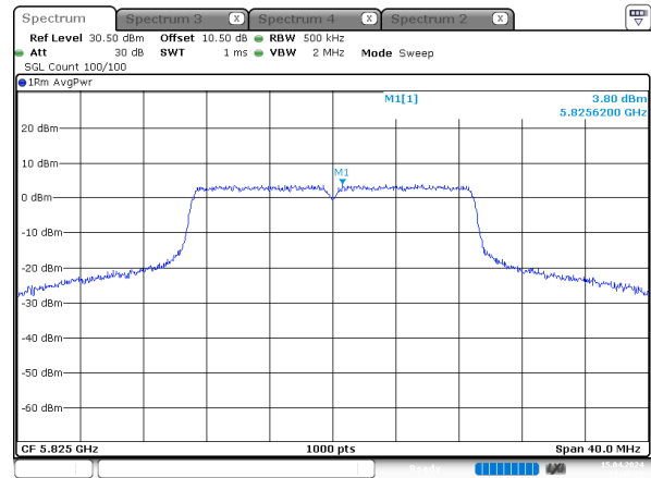
n20_5825MHz_Chain 1
