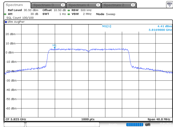
ax20_5825MHz_RU_Full_Chain 1
