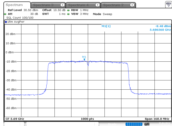
ac80_5690MHz_Chain 1
