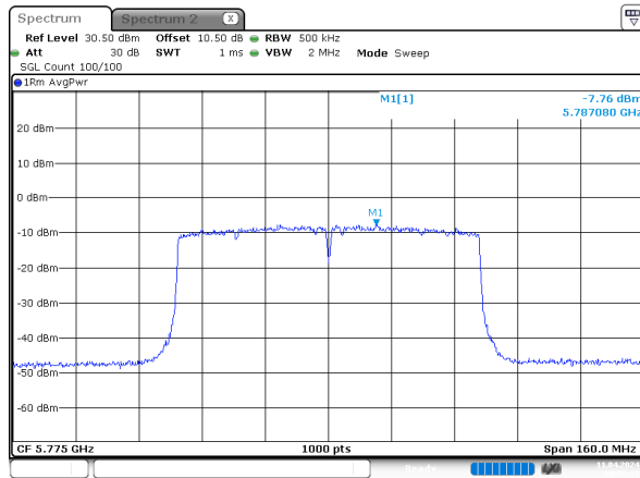
ac80_5775MHz_Chain 0
