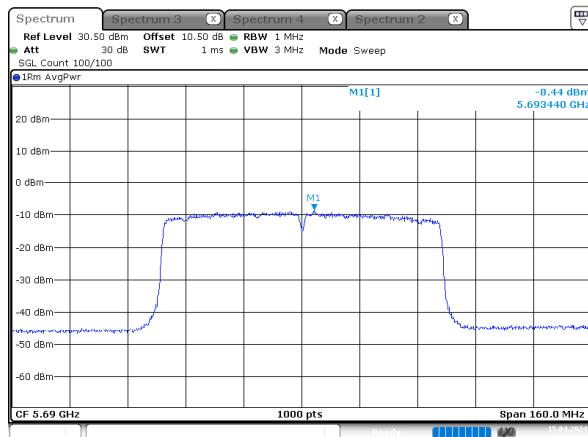
ac80_5690MHz_Chain 2
