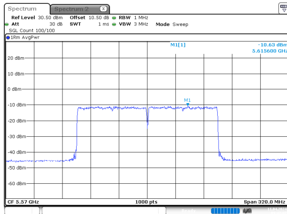
ax160_5570MHz_RU_Full_Chain 0
