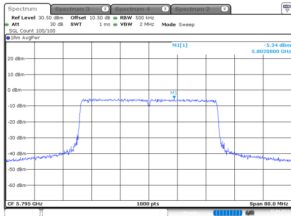
ax40_5795MHz_RU_Full_Chain 2
