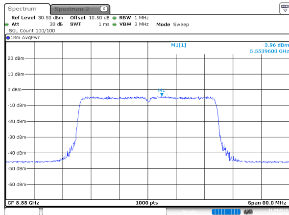
ax40_5550MHz_RU_Full_Chain 0
