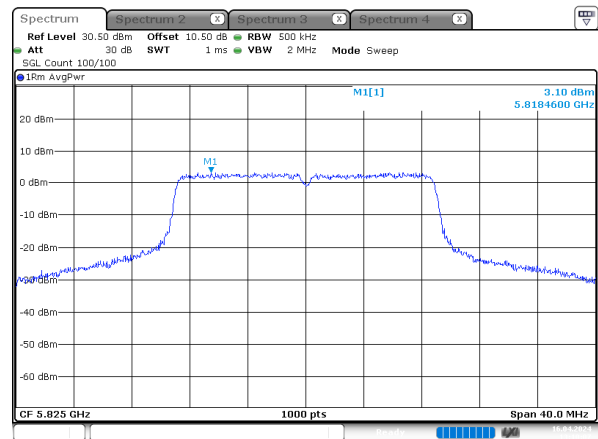
n20_5825MHz_Chain 3
