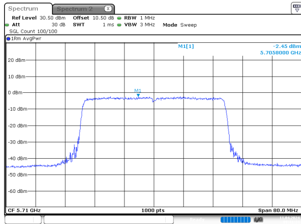
ax40_5710MHz_RU_Full_Chain 0
