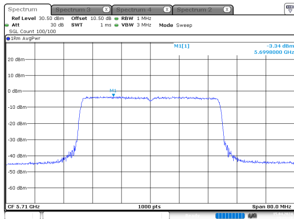
ax40_5710MHz_RU_Full_Chain 2
