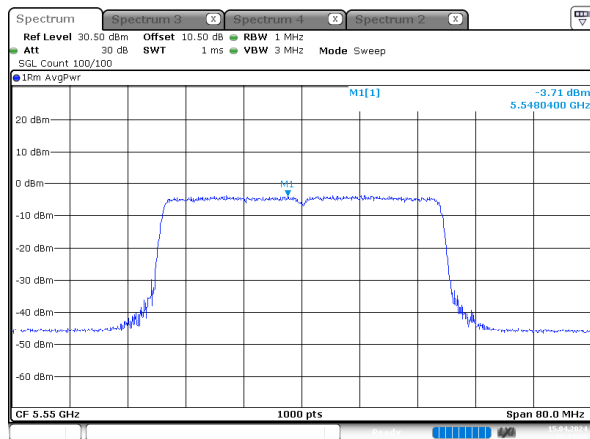
ax40_5550MHz_RU_Full_Chain 2
