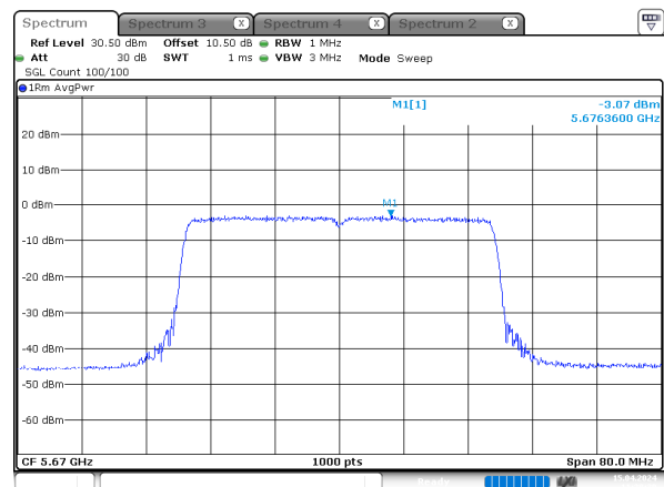
ax40_5670MHz_RU_Full_Chain 1
