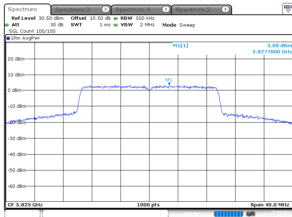
ax20_5825MHz_RU_Full_Chain 2
