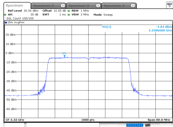
ax40_5550MHz_RU_Full_Chain 3
