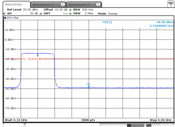
ax40_5190MHz_RU_Full_Chain 3
