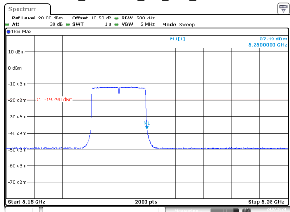
ax40_5230MHz_RU_Full_Chain 1
