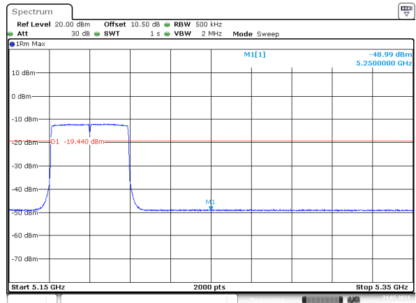
ax40_5190MHz_RU_Full_Chain 1
