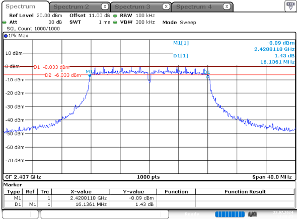
g_2437MHz_Chain 0
