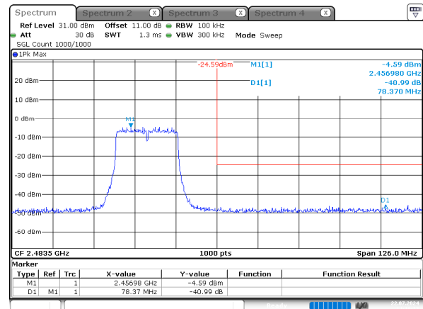
ax20_2462MHz_RU_Full_Chain 1
