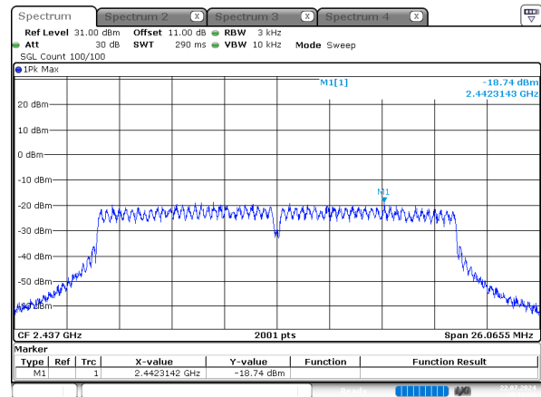
n20_2437MHz_Chain 3
