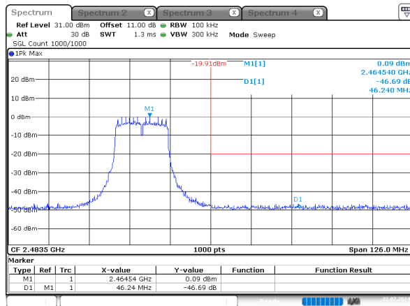
g_2462MHz_Chain 0
