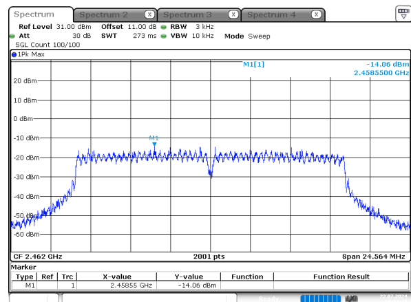
g_2462MHz_Chain 3
