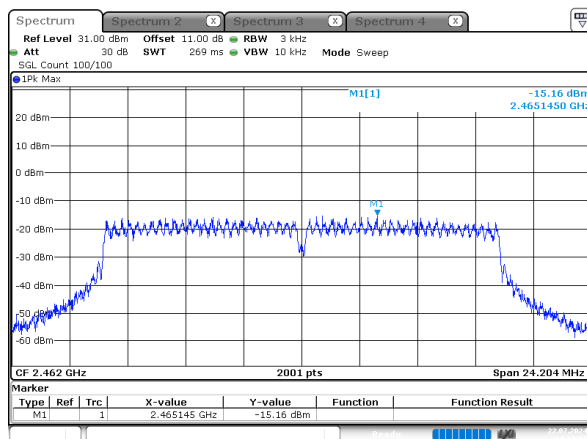
g_2462MHz_Chain 2
