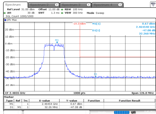
g_2462MHz_Chain 1
