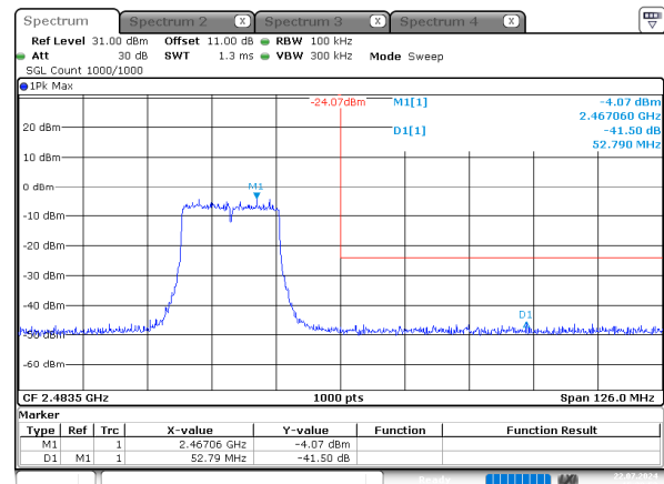
ax20_2462MHz_RU_Full_Chain 3
