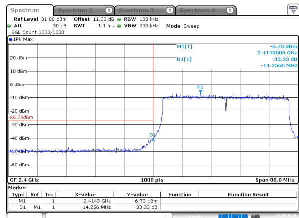
ax40_2422MHz_RU_Full_Chain 1
