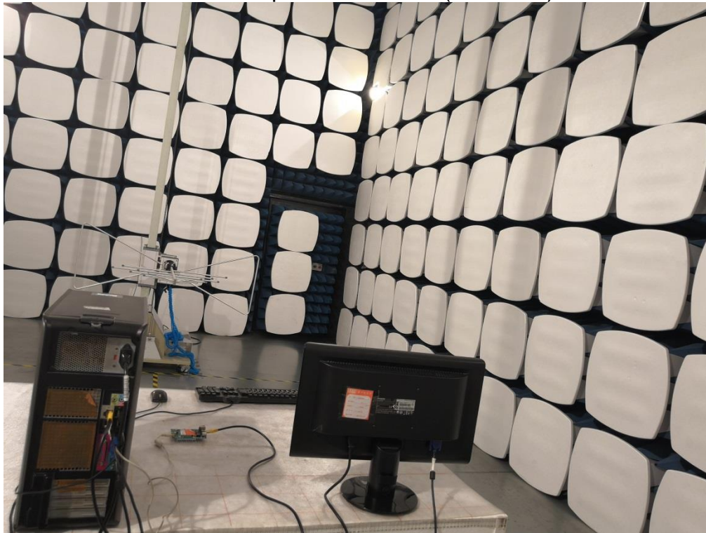
Radiated Spurious Emission(3dBi ANT)
