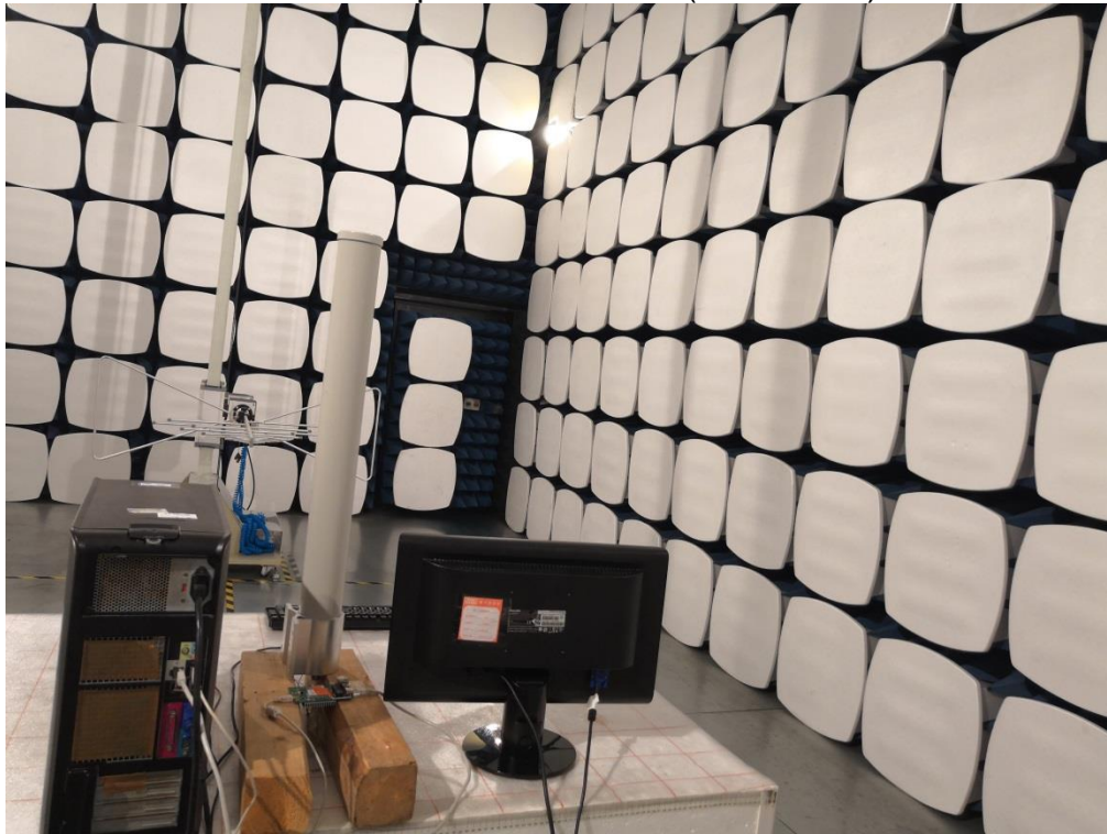
Radiated Spurious Emission(10dBi ANT)
