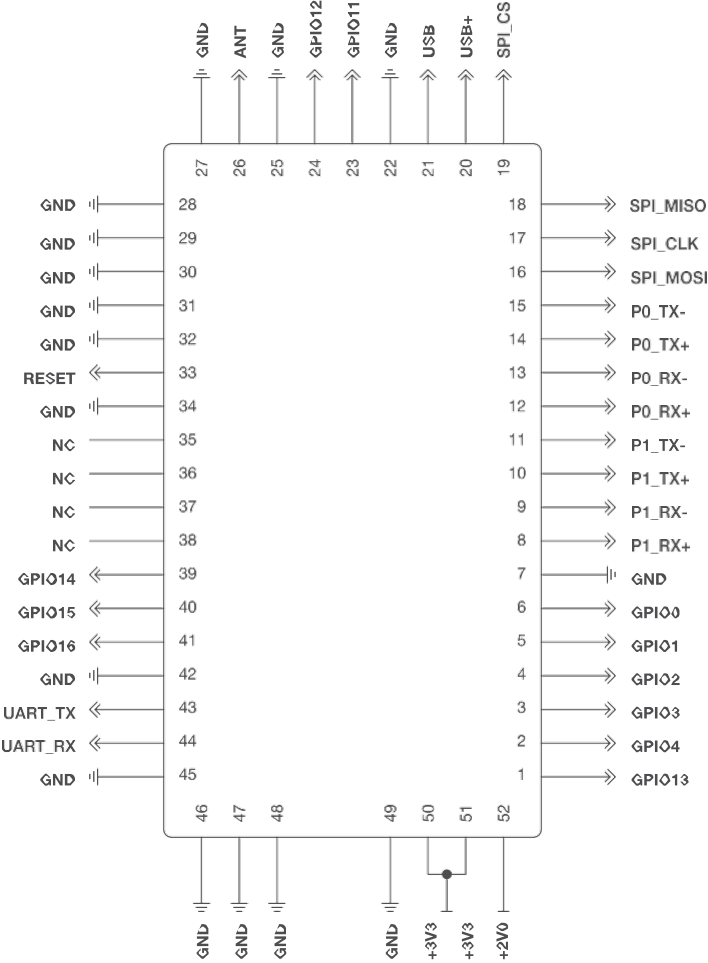
FIGURE 2-1. PIN ASSIGNMENTS
