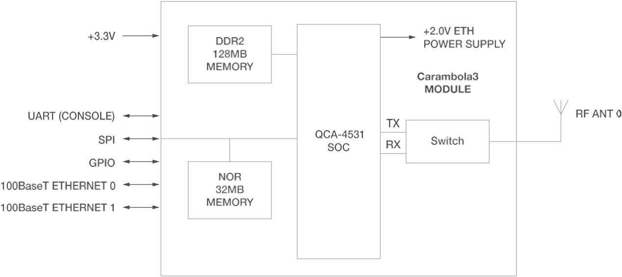
FIGURE 1-1. BLOCK DIAGRAM
