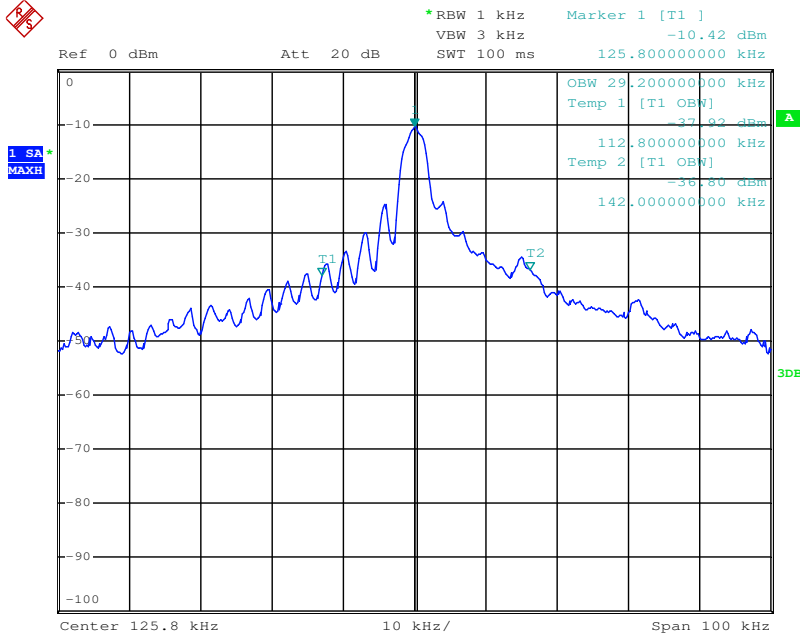
Figure 7.2.2-1: 20dB BW
