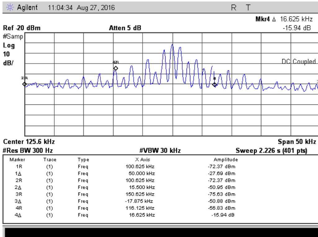
Figure 7.2.2-2: 99% OBW
