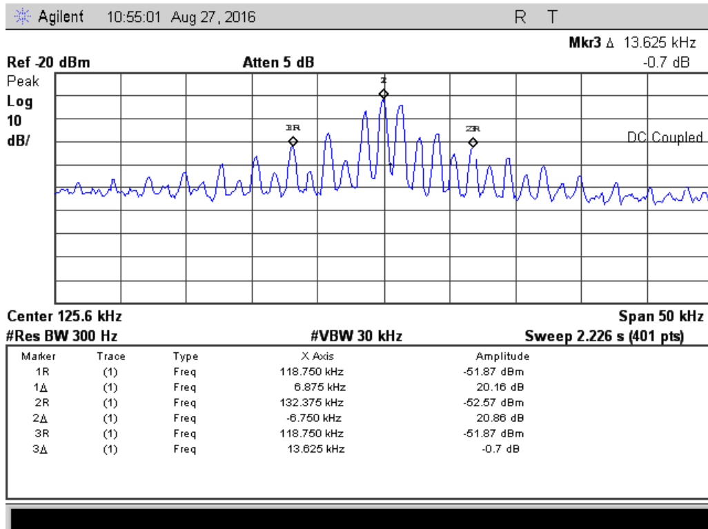
Figure 7.2.2-1: 20dB BW
