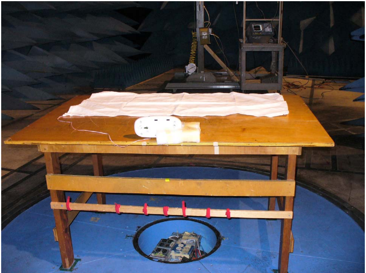
Figure 5: Radiated Emissions – Back View 3
