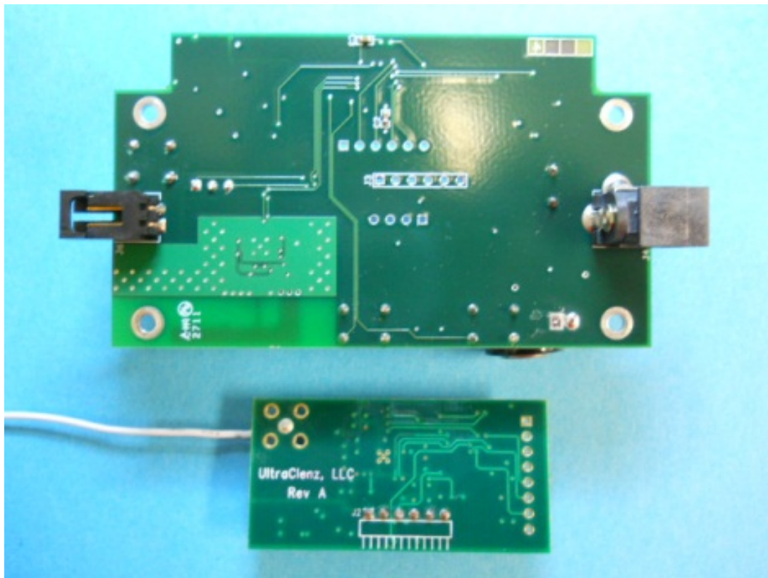
Figure 2: PCB – Bottom View
