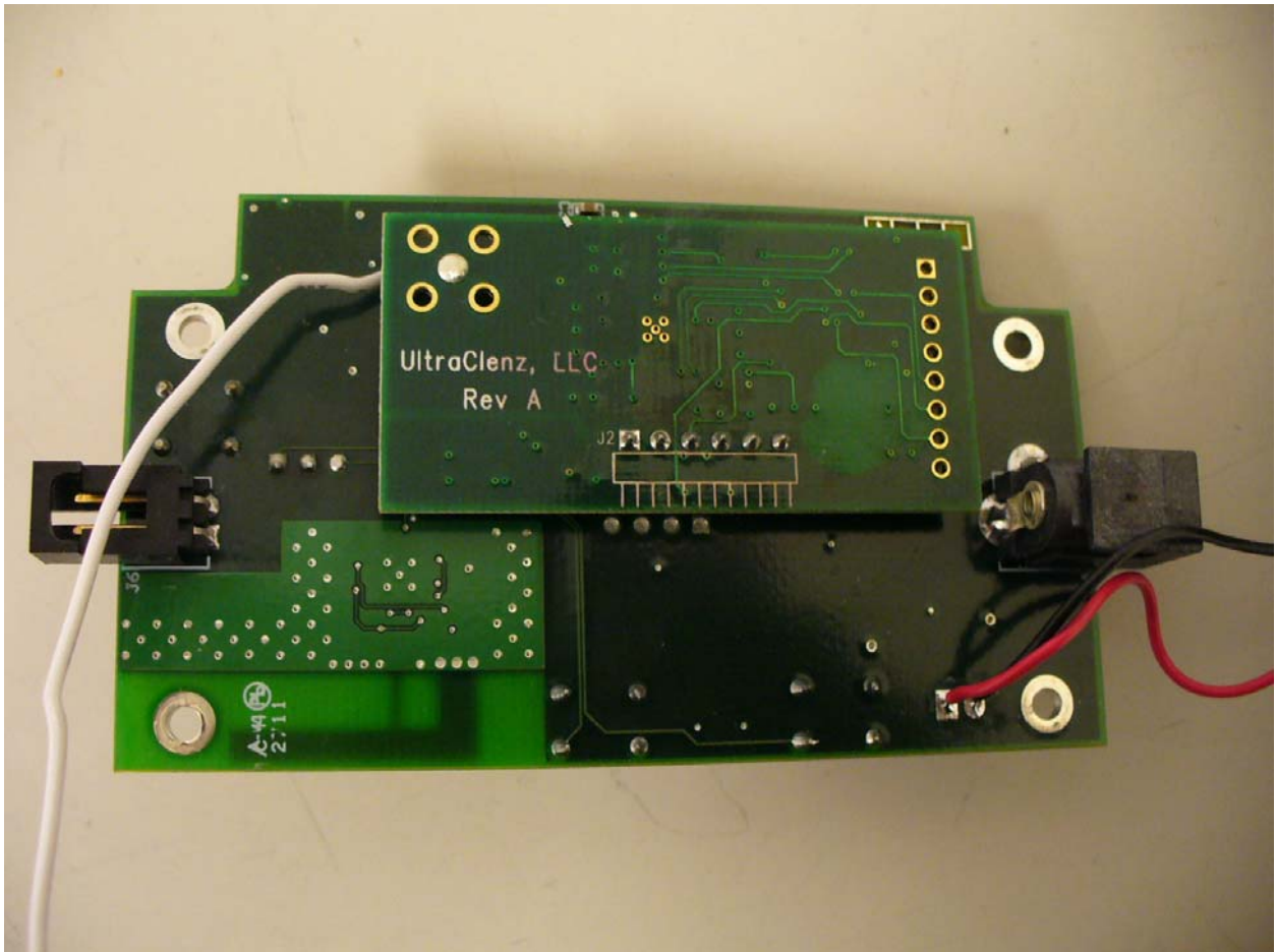
Figure 3: PCB – Assembled View
