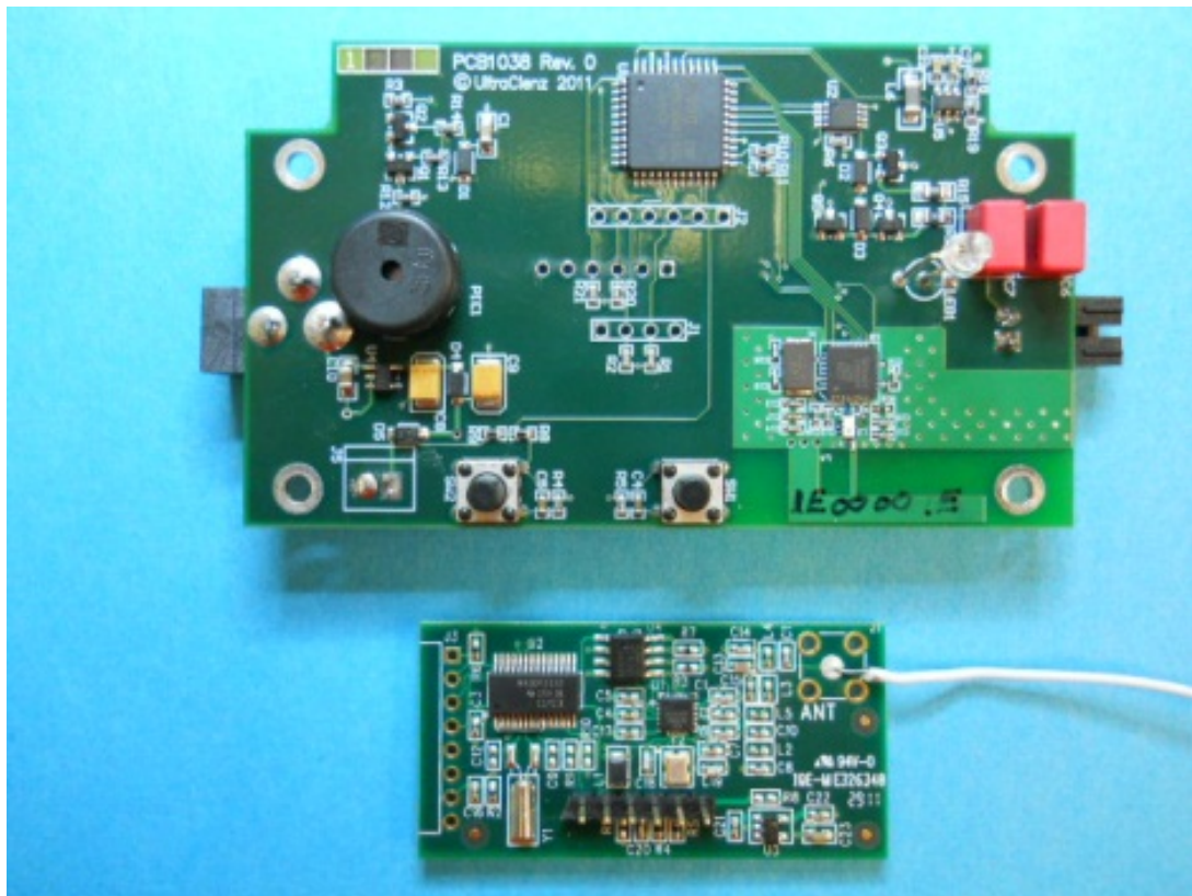
Figure 1: PCB – Top View
