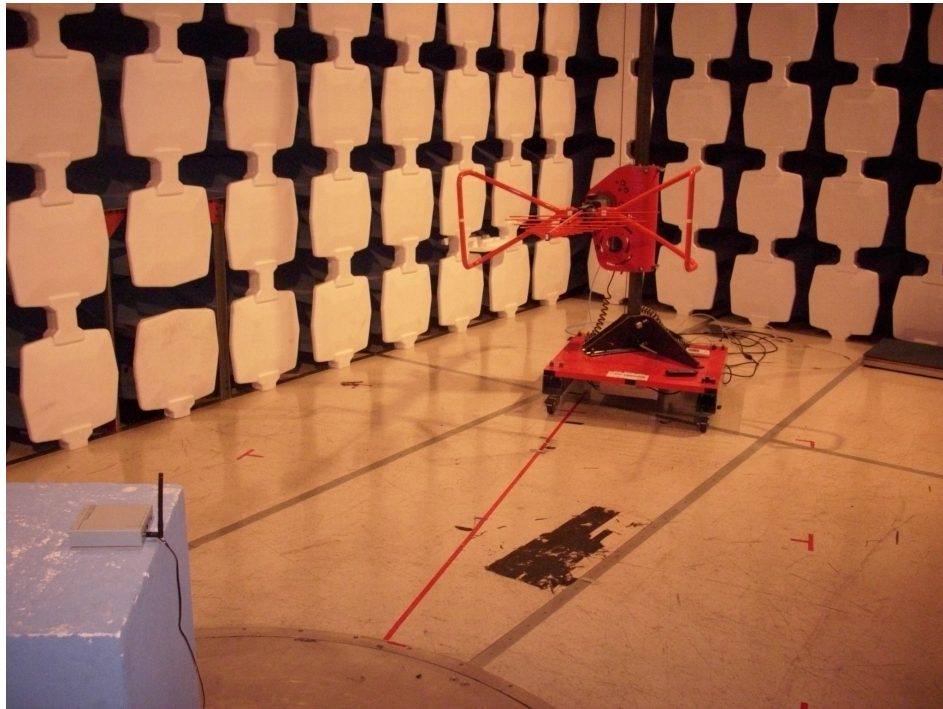
Radiated Measurements – Below 1GHz – Anechoic Chamber
