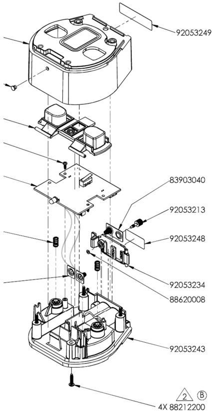
Figure 1 Engineering drawing showing location of 92053249 & 92053248
