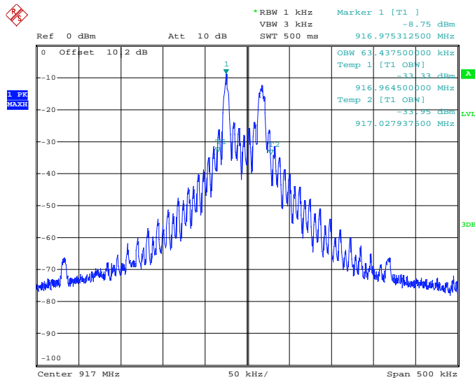
Figure 7.2.2-1: 20dB Occupied Bandwidth
