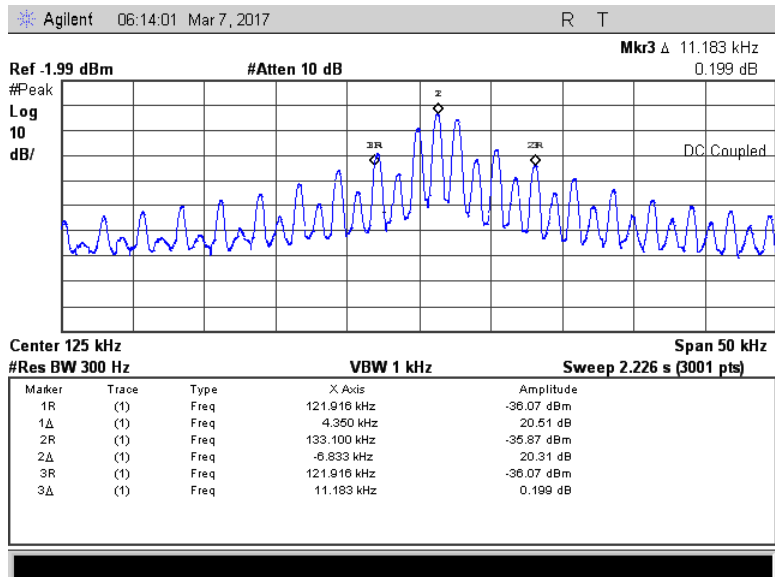
Figure 7.2.2-1: 20dB BW
