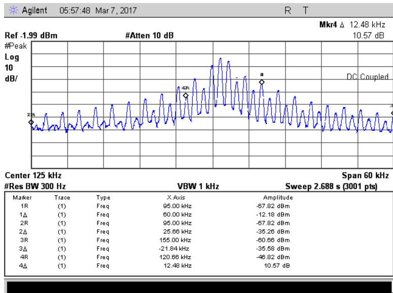
Figure 7.2.2-2: 99% OBW
