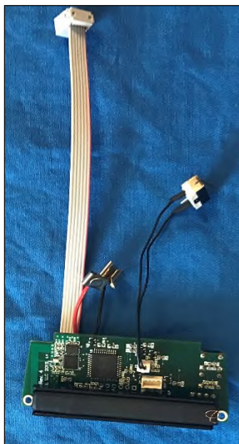
Figure 5: PCB 1053 – Top Side
