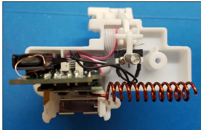
Figure 2: PCB Assembly – Inside Case
