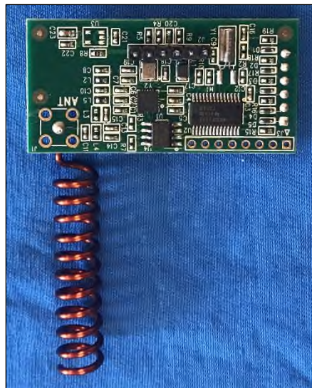
Figure 7: PCB8001 – Top Side
