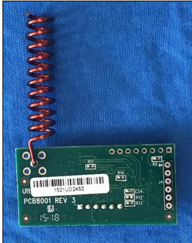
Figure 6: PCB8001 – Bottom Side
