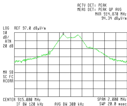
Figure 7. 915.00 MHz Antenna Polarization Vertical
