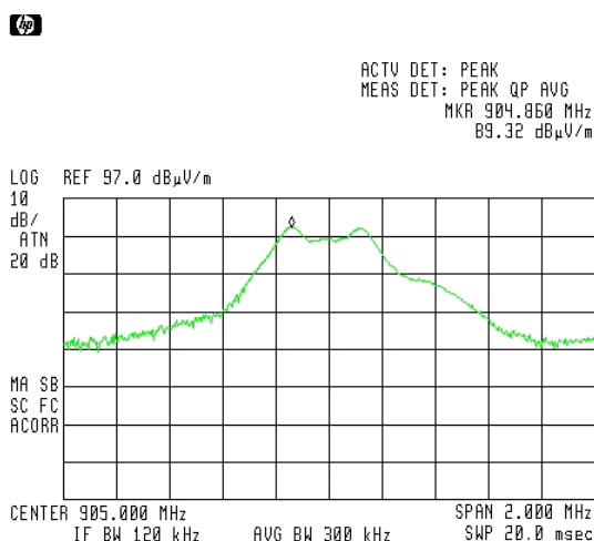
Figure 5. 905.00 MHz Antenna Polarization Vertical
