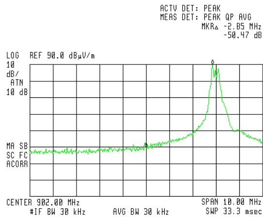
Figure 16. Band Edge Attenuation
