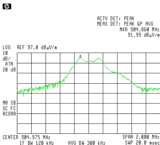
Figure 4. 905.00 MHz Antenna Polarization Horizontal
