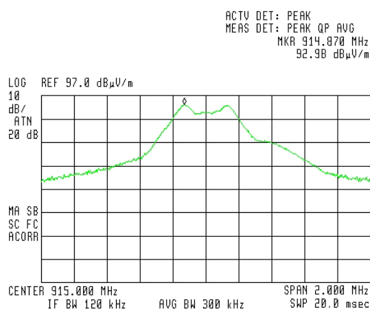
Figure 6. 915.00 MHz Antenna Polarization Horizontal
