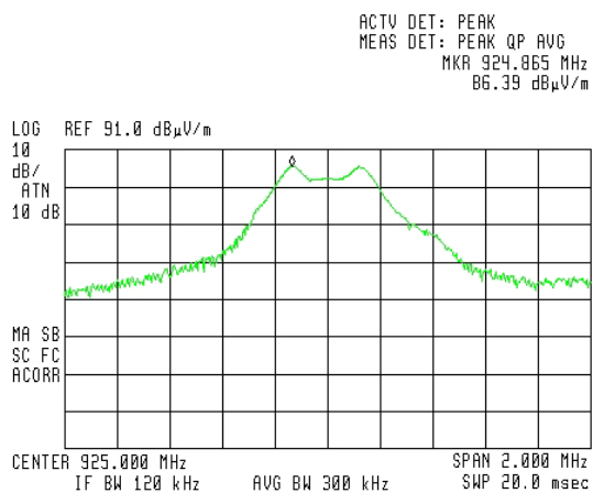
Figure 9. 925.00 MHz Antenna Polarization Vertical
