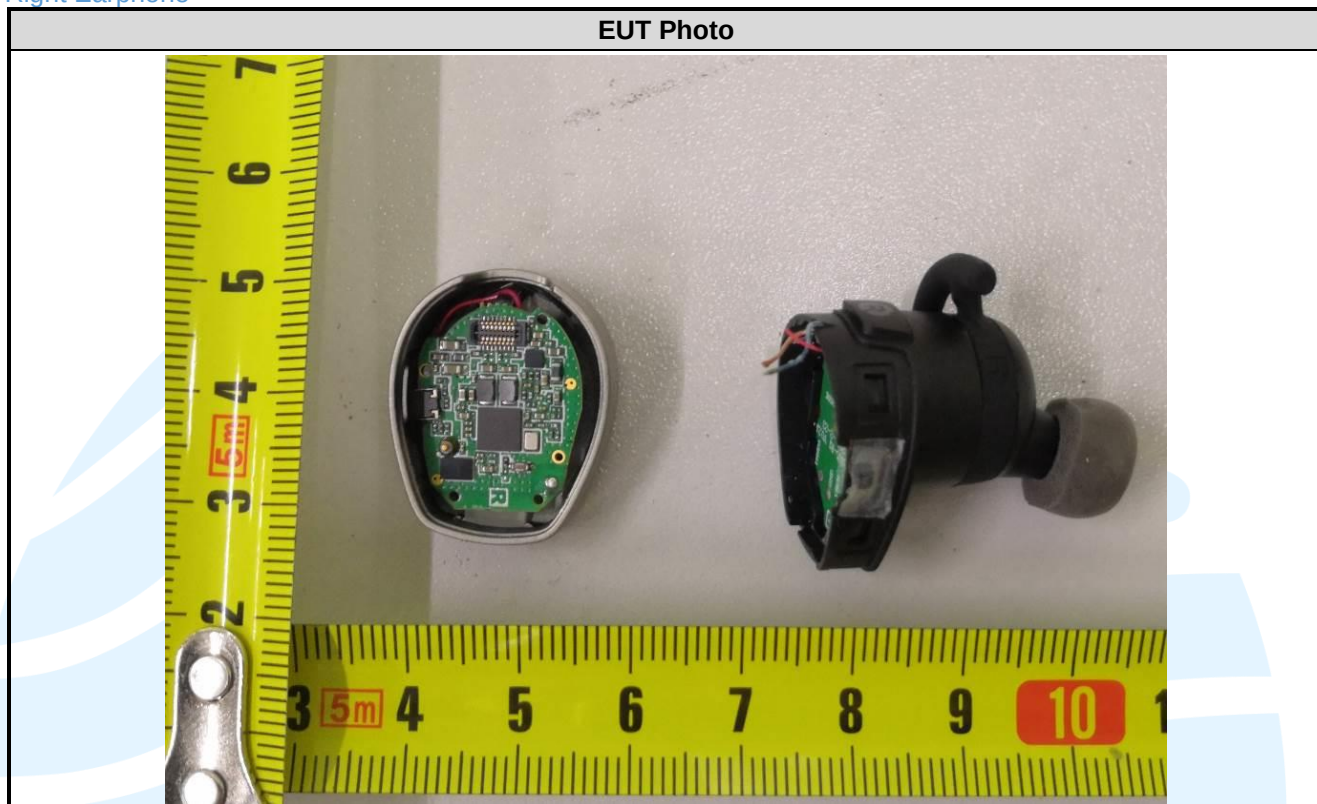
Right Earphone
