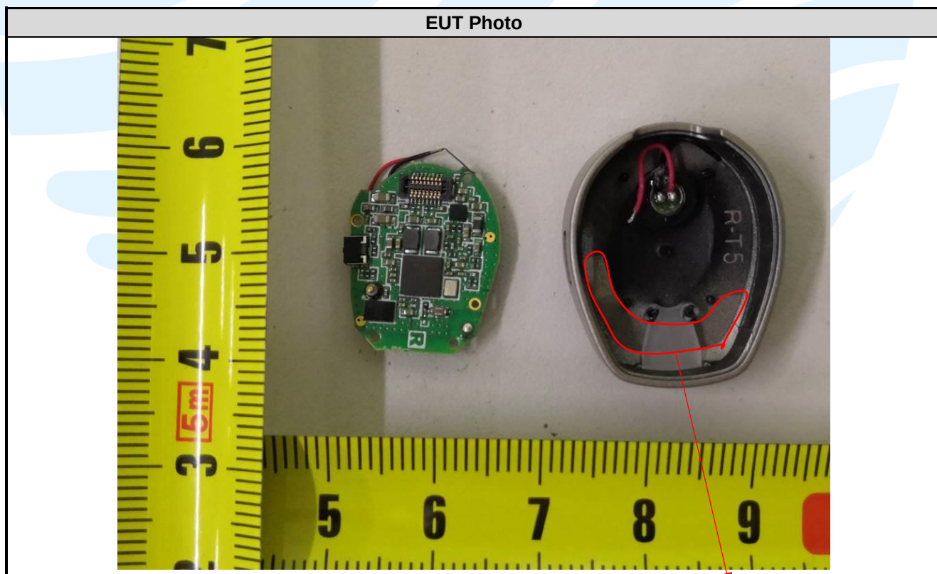
BT Antenna
