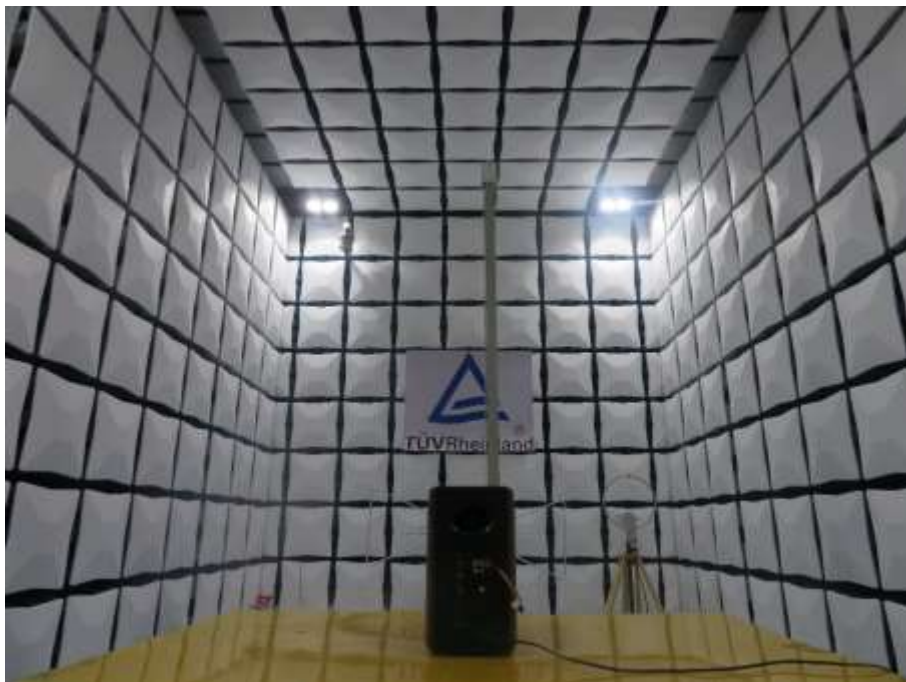
Photograph 4: Set-up for Radiated Spurious Emission, below 1GHz
