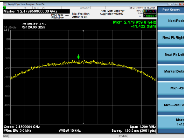
Channel 39 (2480MHz)
