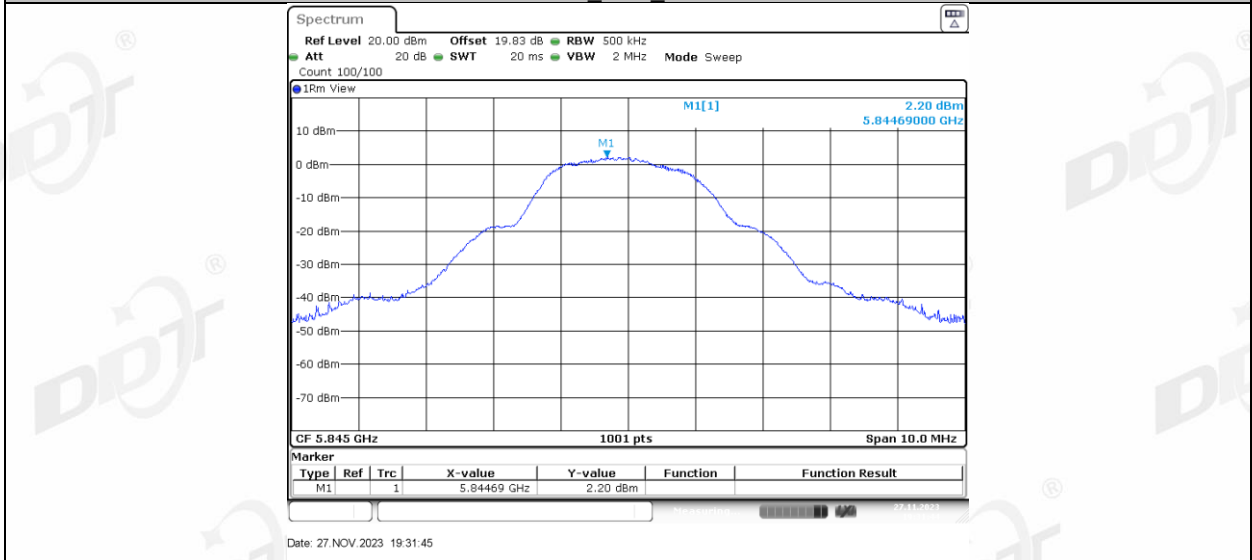
SRD Ant2 5845
