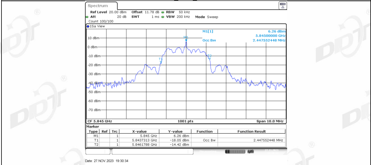
SRD Ant2 5845
