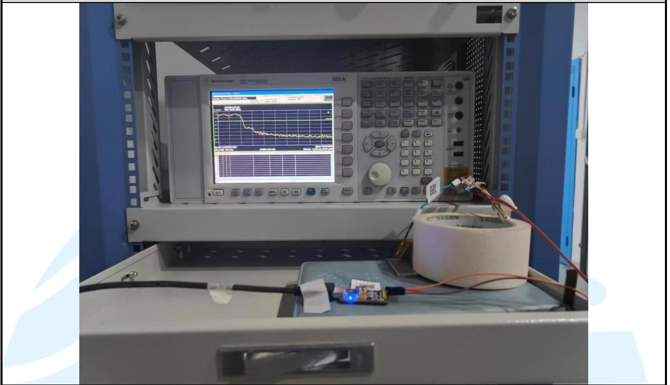
RF Conducted Test Setup_ Left Ear
