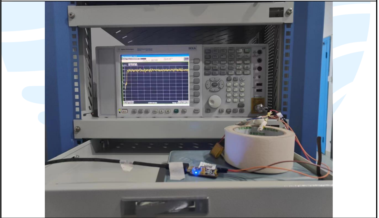
RF Conducted Test Setup_ Right Ear
