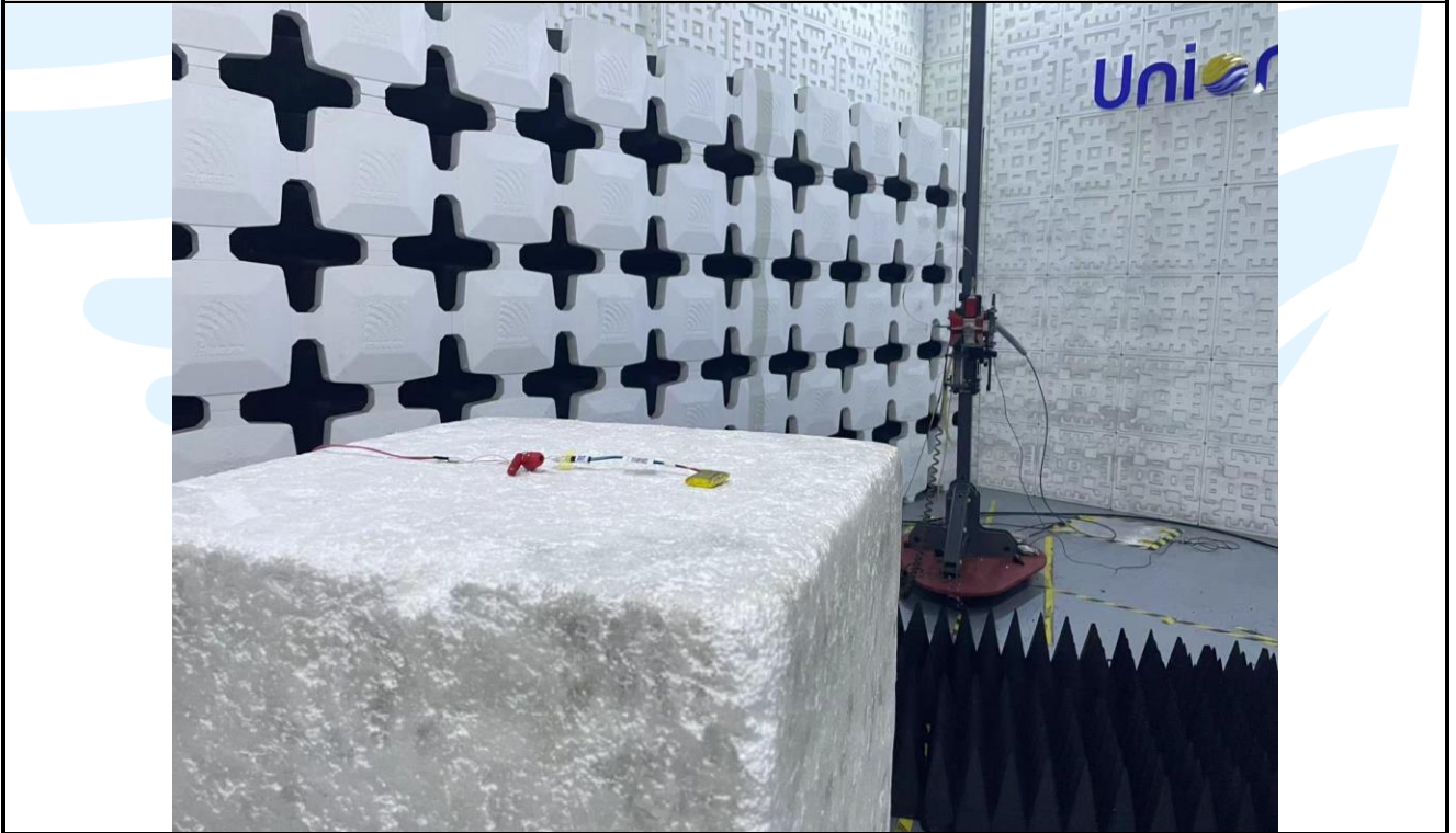
Radiated emission Test Setup (Above 1 GHz) _ Right Ear
