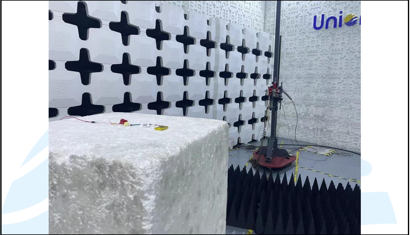
Radiated emission Test Setup (Above 1 GHz) _ Left Ear
