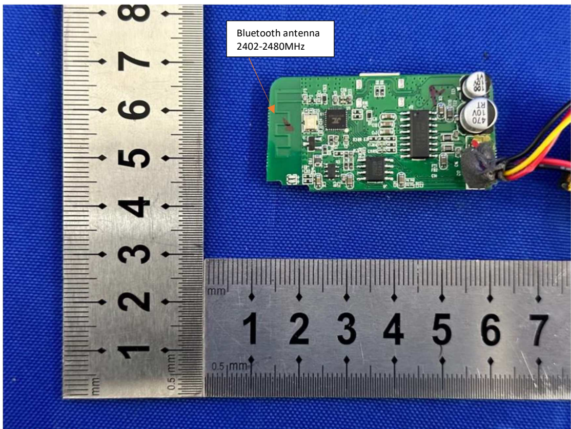
Main PCB view
